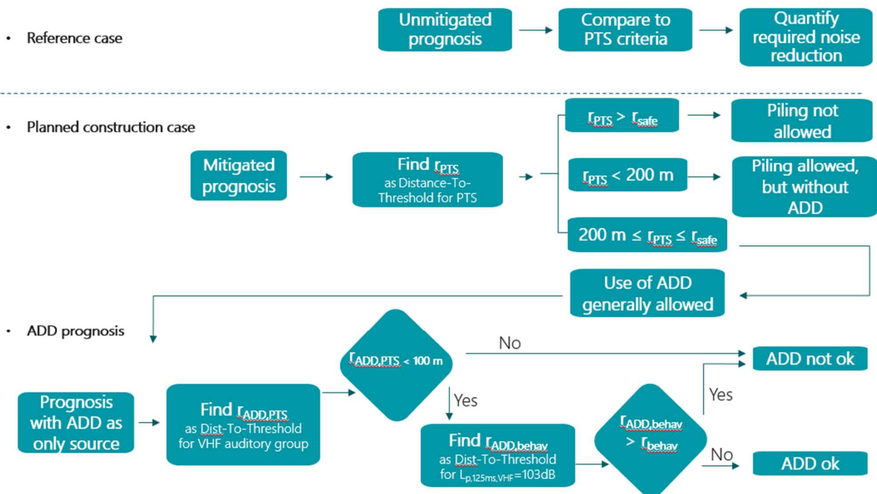
Figure 2: Overview flow diagram for prognosis scenarios.
