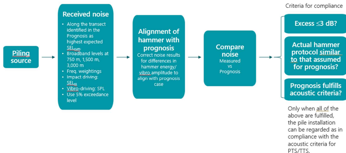
Figure 7: Overview flow diagram for compliance verification.
