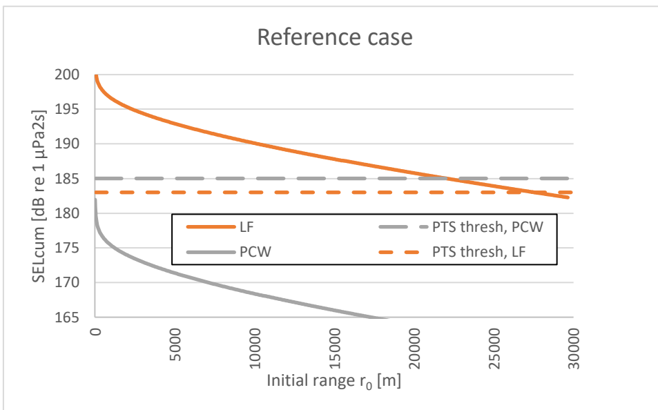
Figure 4: Reference case: Calculated SEL_{cum} as a function of initial distance r_0 for LF and PCW auditory groups. Corresponding PTS thresholds are indicated by dashed lines.
