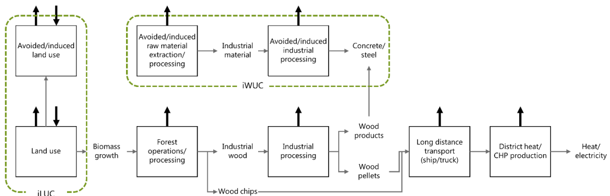
Figure 2.1. Overview of the model framework. Thin arrows represent material flows, while thick arrows represent material and energy flows.
