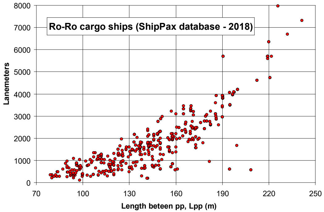
Figure 44 Lane meters for Ro-Ro cargo ships as function of length between pp, Lpp
