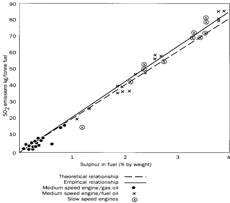
Figure 64 Relationship between fuel sulphur content and SO 2 emissions for marine diesel engines (Lloyds Register of Shipping, 1995)
