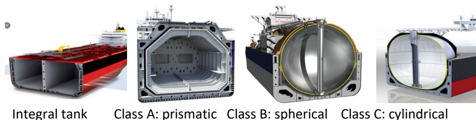
Figure 23: Different tank classes. The most cost-efficient onboard storage of ammonia seems to be class C (pressurized tanks) (Topsoe, 2020).
