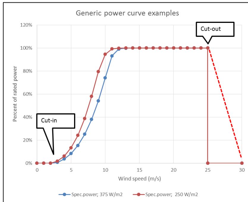
Figure 2 Turbine power curves (Information's from expert workshop held by DEA 27-4-2015). Specific power values refer to e.g. 3 MW with 124m rotor diameter (250 W/m2) and 3 MW with 101 m rotor diameter (375 W/m2)
