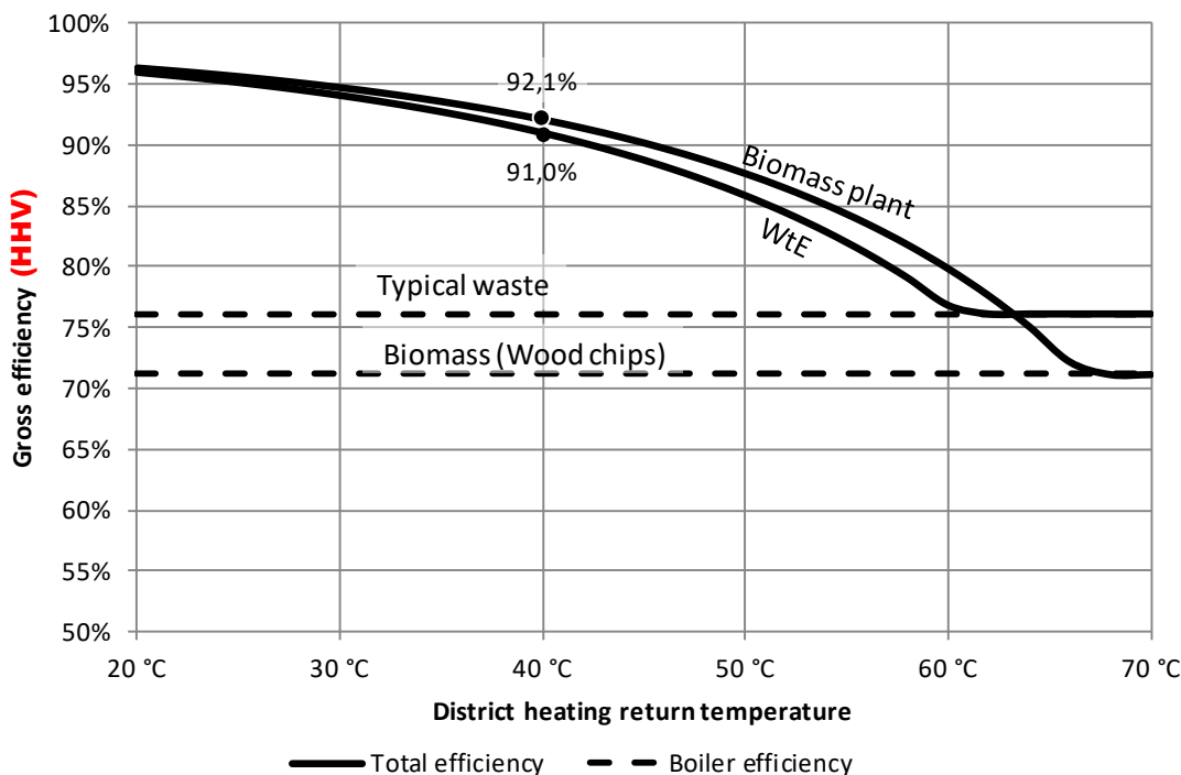
Figure 9. Total HHV-based efficiency estimate for WtE plants 7 and biomass plants 8 given varying DH return temperatures [5] – or temperature of the cold media of a heat pump.
