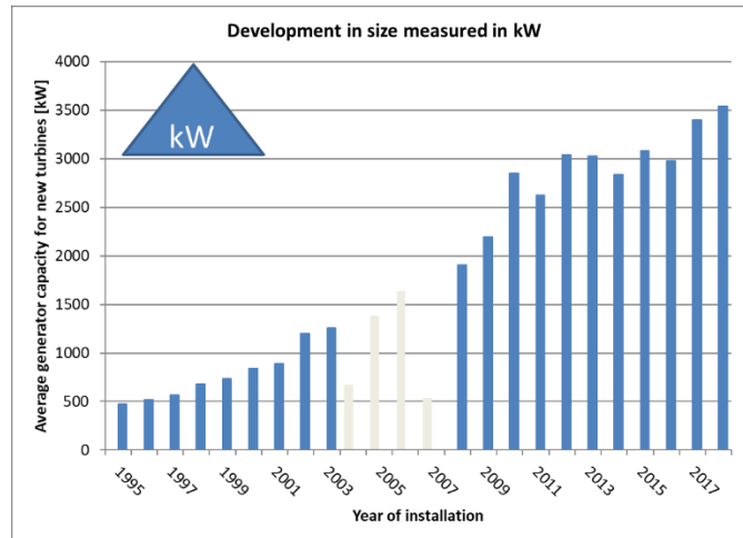
Figure 7 Average generator capacity for new turbines (rated power > 25 kW) [3]
