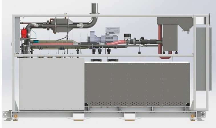
Figure 1: SOFC unit from Sunfire for combined heat and power for commercial use [9].
