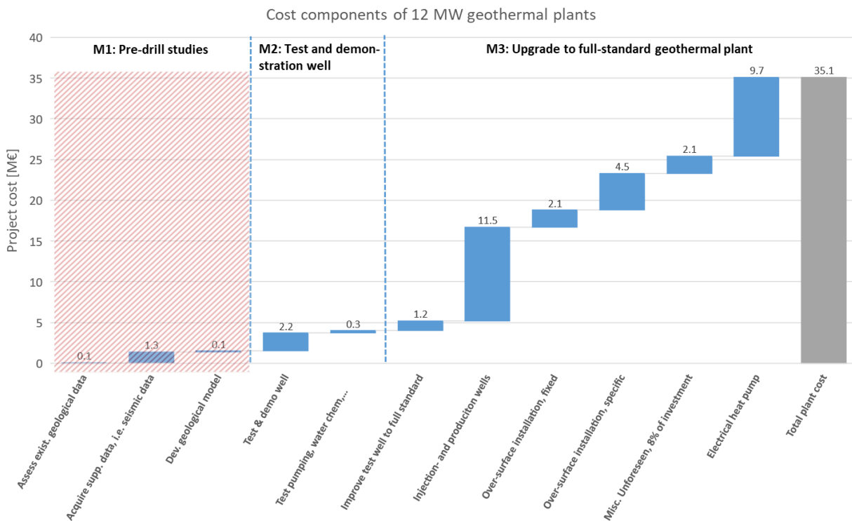
Figure 10 Cost components of a 12 MW geothermal plant 1.a - 1,200 m reservoir with electrical heat pump. Definition of milestones (M1-3) given in [14].
