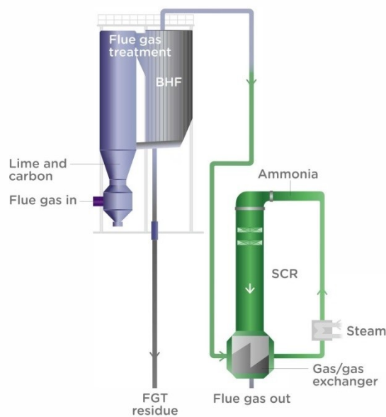
Figure 6 Flue gas treatment system (dry/semi-dry) including reactor with injection of hydrated lime, a bag house filter and an SCR system with gas/gas heat exchanger, steam reheater, ammonia injection and catalyst.
