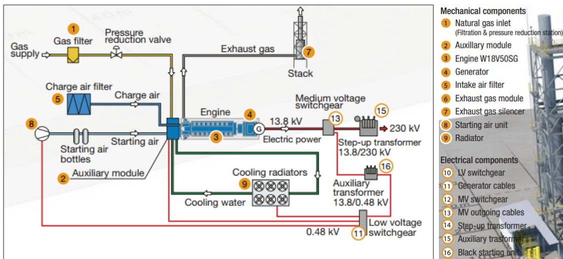
Figure 1 Large engine power plant scheme [16].
