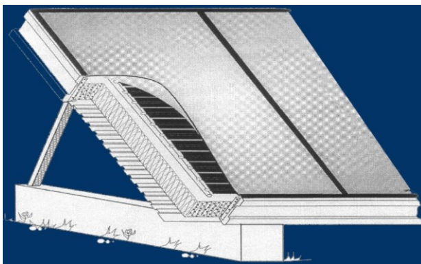
Figure 1 Basic principle of a flat plate solar collector
