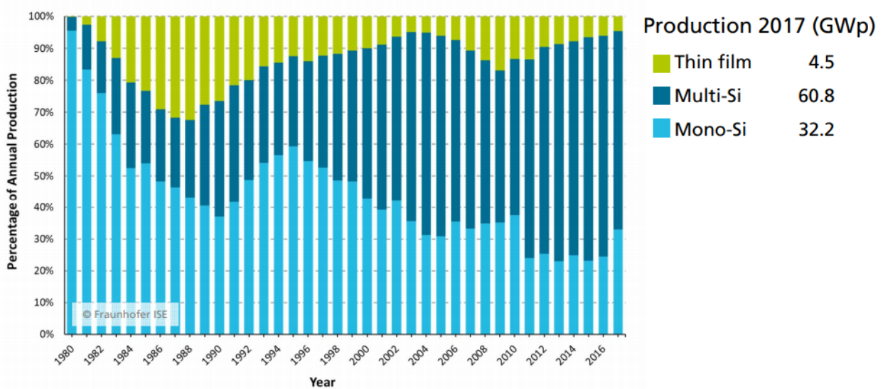
Figure 24 Historical market shares of different cell technologies (Ref. 9).
