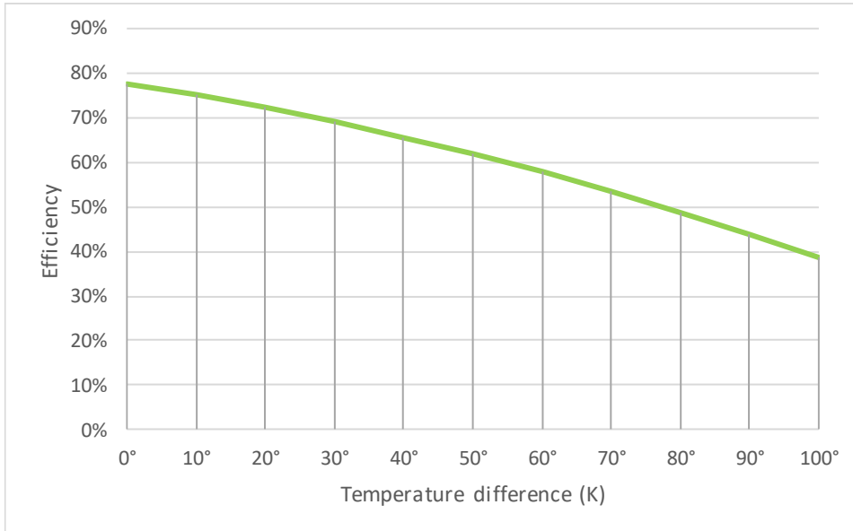
Figure 3 Efficiency as a function of temperature difference. (Based on data from [8], example with G=1.000 \text{ W/m}^2 , \eta_0=0.777 , a_1=2.41 , a_2=0.015 ) 23
