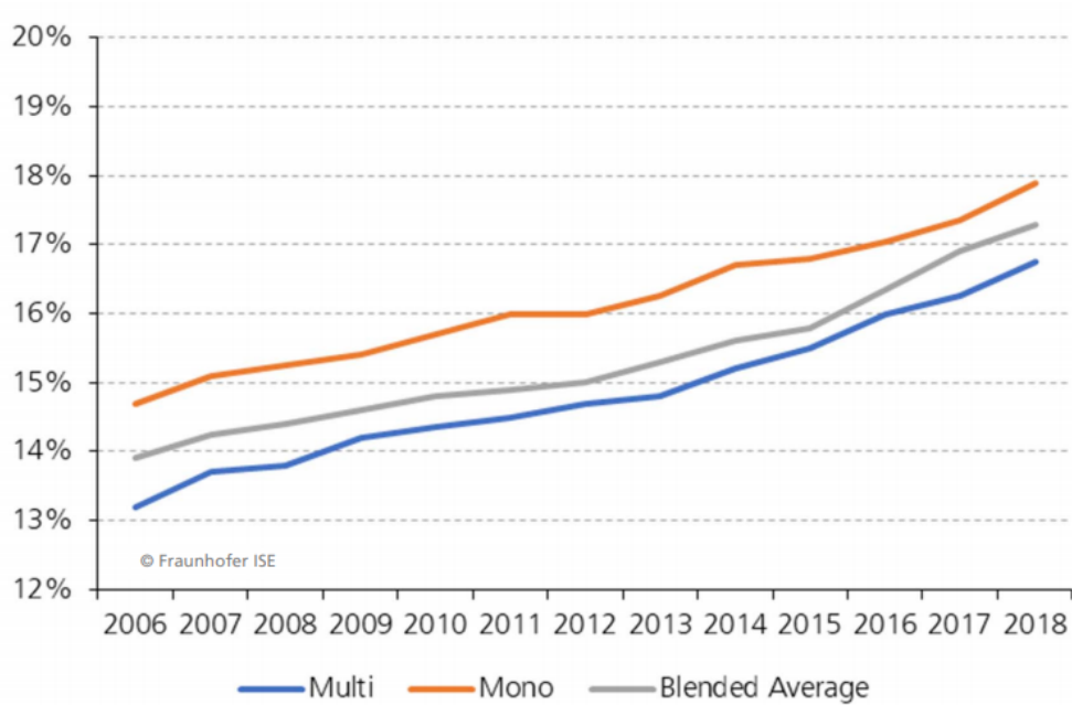
Figure 32 Efficiencies of different cell types (Ref. 9).
