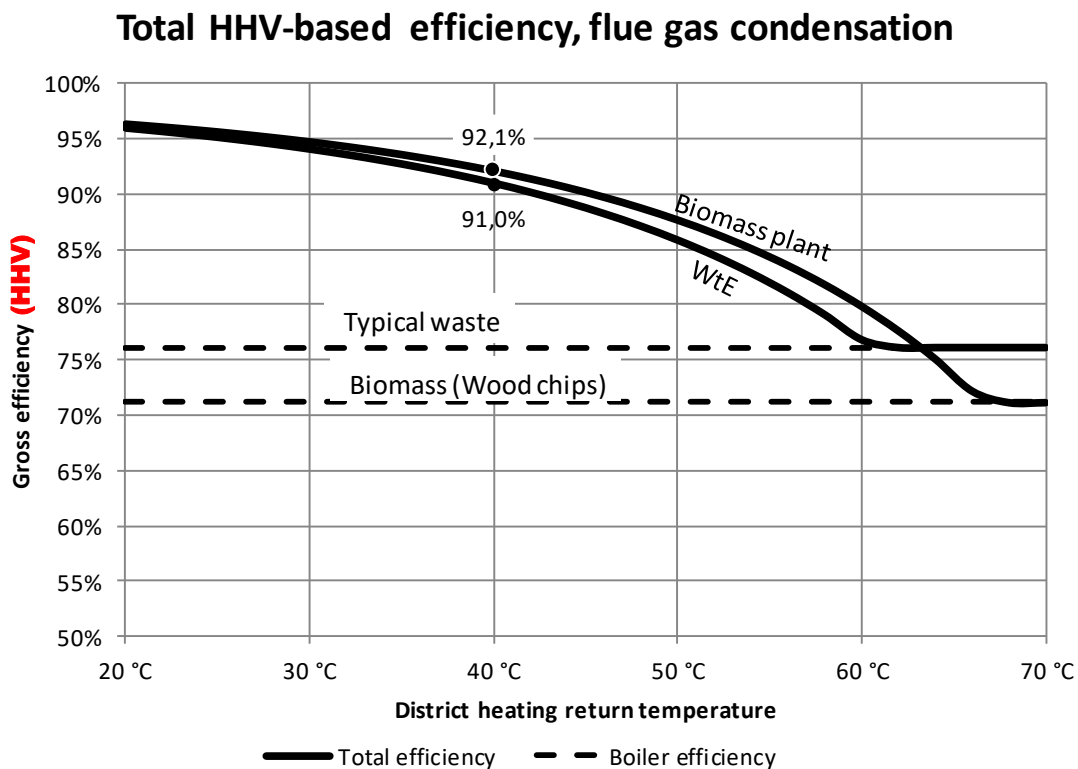
Figure 9. Total HHV-based efficiency estimate for WtE plants and biomass plants given varying DH return temperatures [5] – or temperature of the cold media of a heat pump.
