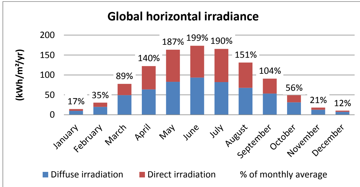
Figure 1: Monthly sum of global irradiance on a horizontal surface averaged over 25 Danish measurement stations over a period of 10 years (2001-2010) (Ref 4). The split between direct and diffuse components of the irradiation is based on the Meteonorm '97 dataset for Copenhagen. Percentage of average monthly is also shown.
