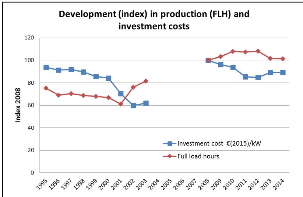
Figure 16: Development (index 2008=100) in investment cost (2015 price level) and average production (full load hours) for onshore turbines > 0.5 MW by installation year based on 2014 production [3, 16, 2]
