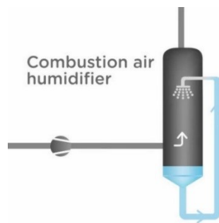
Figure 6 Combustion air humidifier, where water heated by a low-temperature source is evaporated into the combustion air flow.
