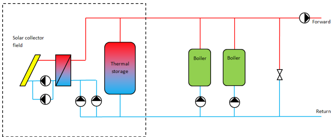
Figure 5 Schematic drawing of a possible system integration of solar district heating [5].
