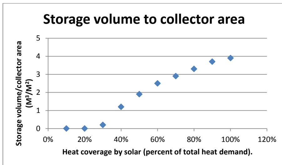
Figure 12 Ratio of seasonal storage volume to collector area (y-axis) as a function of solar heat coverage [4] and [5].
