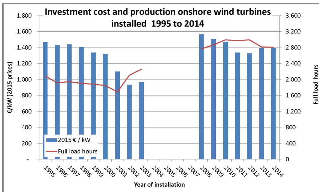
Figure 15: Development in investment cost (2015 price level) and average production (full load hours) for onshore turbines > 0.5 MW by installation year based on 2014 production 12 [3, 16, 2]
