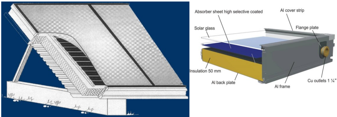
Figure 2 Basic principle of a flat plate solar collector.
