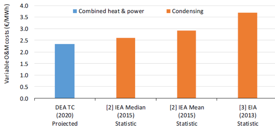
Figure 4: Variable O&M cost (2015€/MWh). The year in ( ) indicate the year of the projection or statistic.
