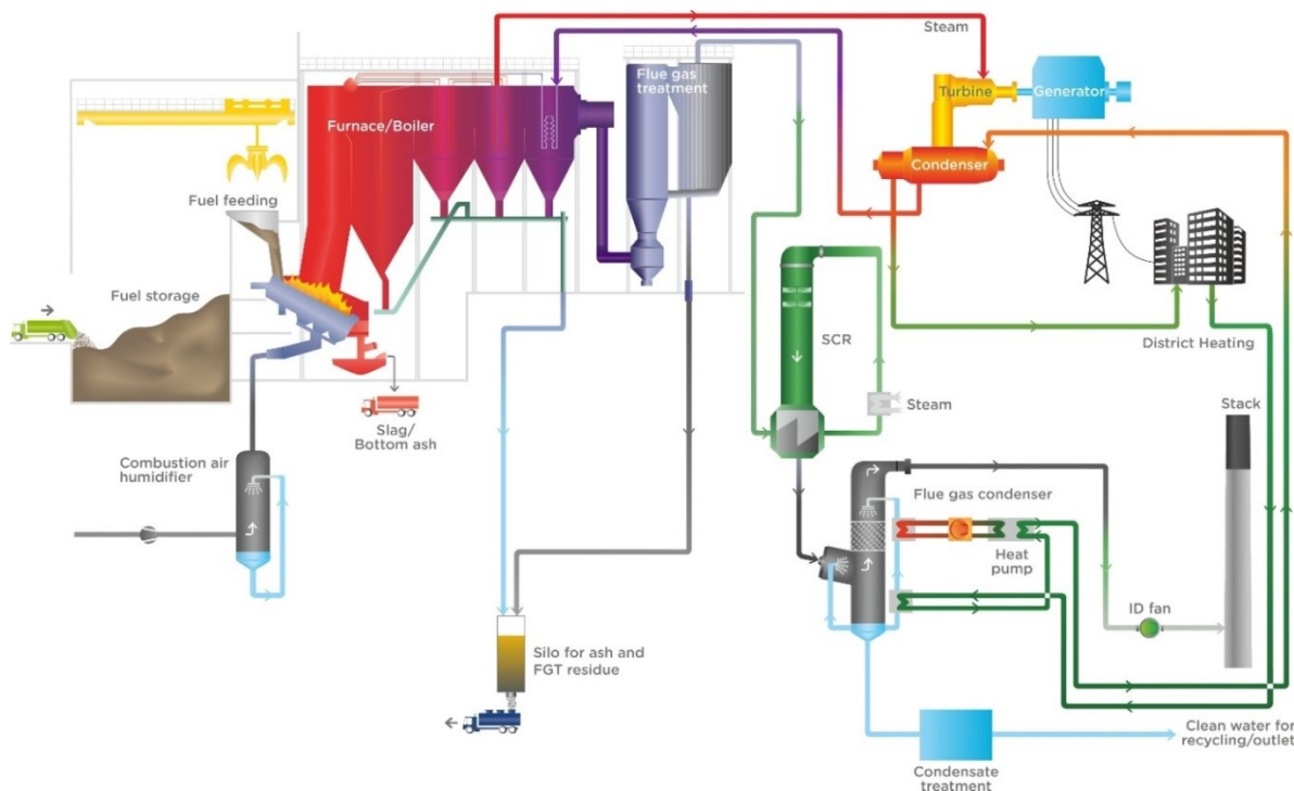
systems of a CHP (or Heat only) facility, example WtE CHP facility
