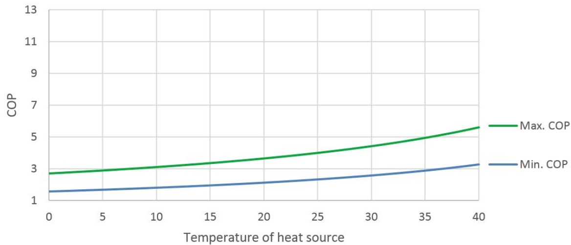
Figure 5: COP values of compression heat pump heating water from 60 to 90° C. For a heat source @ 0° C that is cooled to -5° C, typical COP values will be 1.6-2.7 rising to 3.2-5.6 for a heat source @ 40° C that is cooled to 35° C [1].
