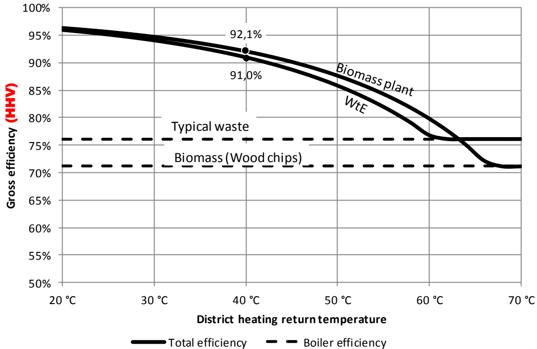
Figure 7. Total HHV-based efficiency estimate for WtE plants 7 and biomass plants 8 given varying DH return temperatures [5] – or temperature of the cold media of a heat pump.
