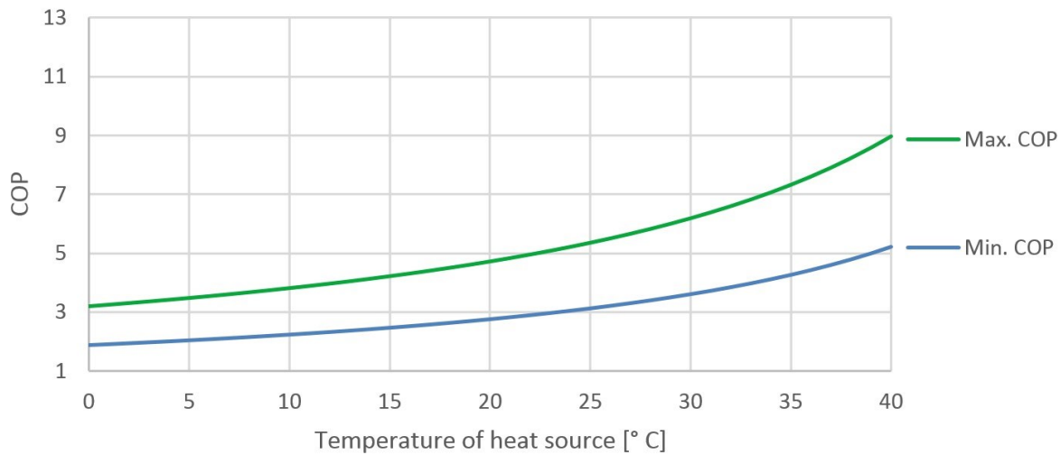
Figure 4: COP values of compression heat pump heating water from 45 to 75° C. For a heat source @ 0° C that is cooled to -5° C, typical COP values will be 2.0-3.1 rising to 5.0-9.0 for a heat source @ 40° C that is cooled to 35° C [1].
