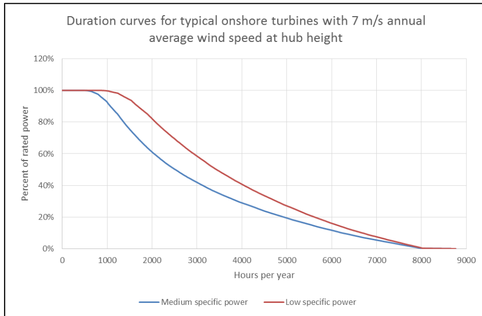
Figure 3: Duration curve for typical modern onshore wind turbines (> 2 MW) located in Denmark (DTU International Energy Report - Wind Energy, 2014). The two curves are based on the V117 3.3 MW (307 W/m 2 ) and V126 3.3 MW (265 W/m 2 ) wind turbines.
