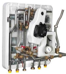
Figure 16: Metroterm 3 20kW direct DH unit [7]
