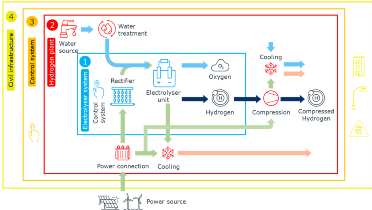
Figure 2 Flow diagram of major streams and components in a hydrogen plant.
