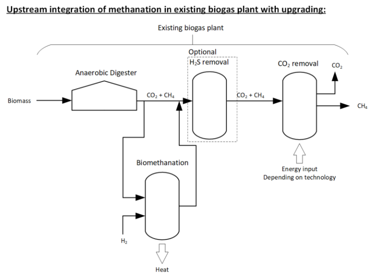
Figure 4: Integration examples of biomethanation (ex-situ) in existing biogas plants. Data from some suppliers indicate that grid level biomethane could be achieved directly after the biomethanation reactor, meaning the CO 2 removal unit and H 2 S unit could be optional and omissible to save costs. This has been proven in demonstration scale. Water vapor is also removed prior to injection the methane on the grid (not shown).
