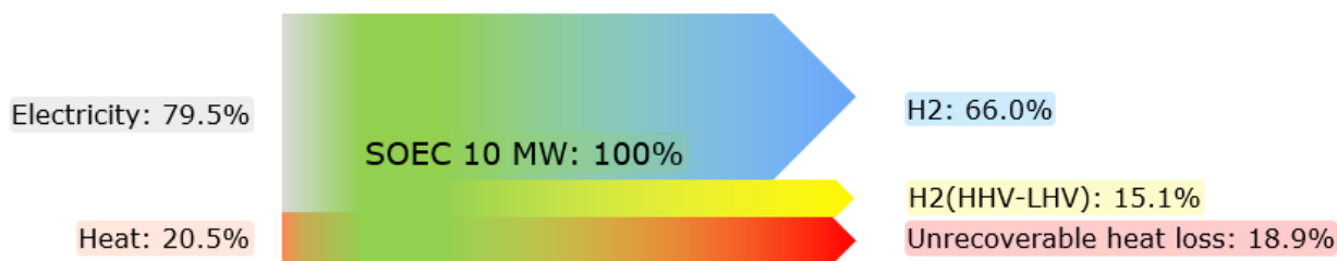
Figure 11 The energy inputs and outputs of an SOEC (2020, 10 MW hydrogen plants). Data is derived from Ramboll references.
