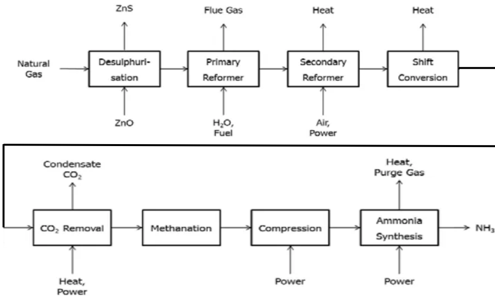
Figure 2: Conventional ammonia plant
