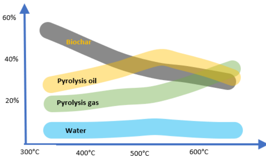
Figure 2. Approximative typical distribution of products depending on pyrolysis temperature. Other factors than temperature also have an impact of this distribution, e.g. particle size, raw material and type of technology used (5).
