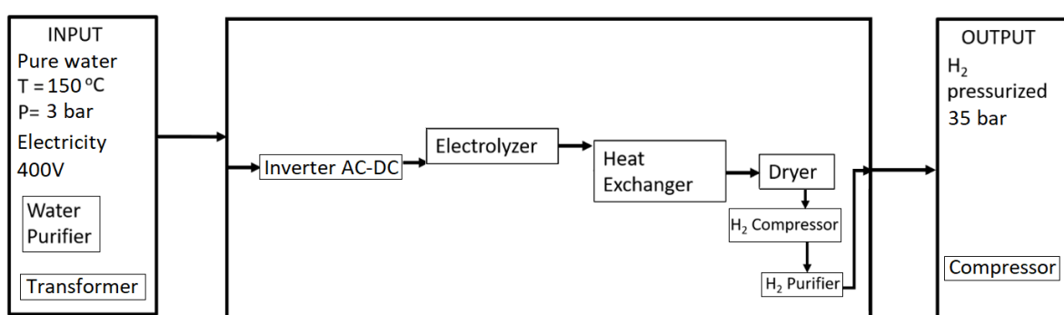
Figure 6: A sketch of an electrolysis system for SOEC.
