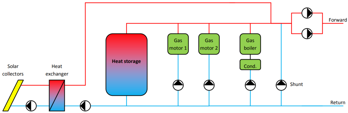
Figure 1: Principal scheme of the hydraulic integration of a large scale water tank in a simple district heating system [6].
