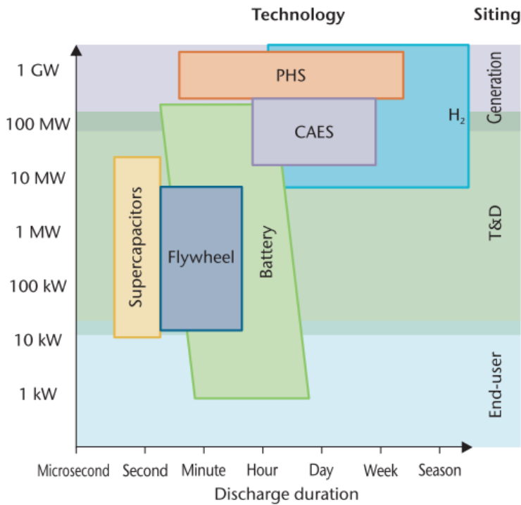
Figure 4: Electricity storage technologies [5]
