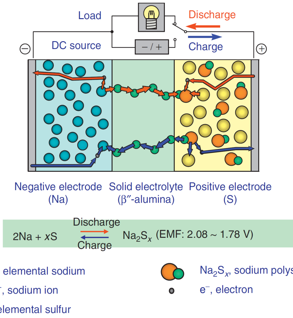
Figure 2: Graphical schematic of the reaction process and the full cell reaction. EMF: electromotive force. [4]
