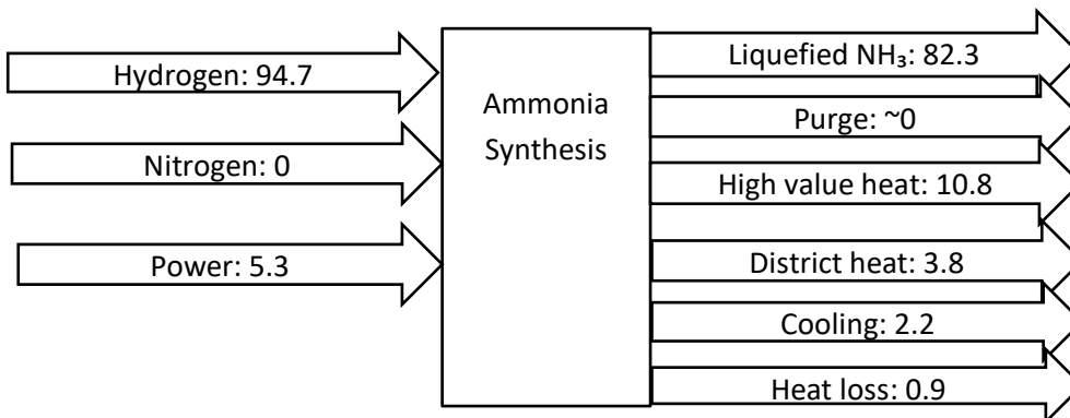
Figure 12: Overall energy balance of the ammonia synthesis. The electrolysis unit is covered in [4] and power required for the ASU is listed in Table 3-1.
