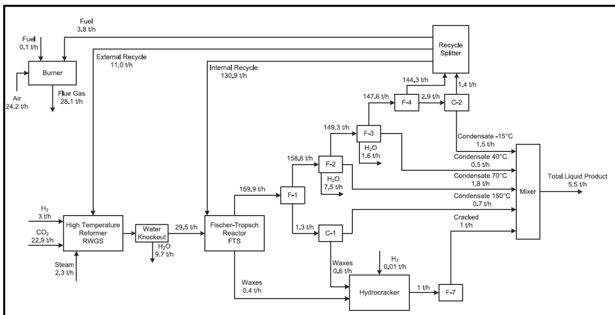
Figure 3: Mass Balance
