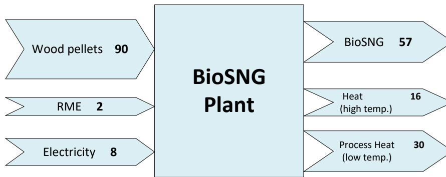
Figure 1 Example of Energy balance. All inputs sum up to 100 units.
