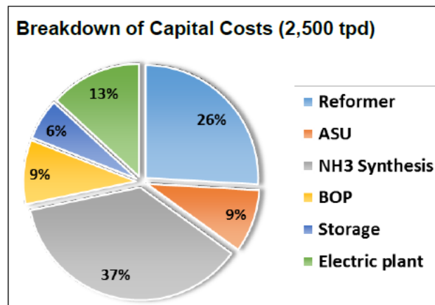
Figure 15. Cost split on main systems in a conventional \text{NH}_3 plant from Linde [10]. Reformer, electric plant (power plant) and some balance of plants (BOP) will disappear for a green \text{NH}_3 plant. Cost of green \text{NH}_3 plant (excl. electrolysis unit and ASU) is therefore taken as 54% of conventional plant, based on all obtained data.
