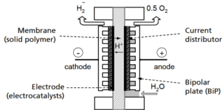
Figure 1: Principle of a PEMEC. Adopted from [13]
