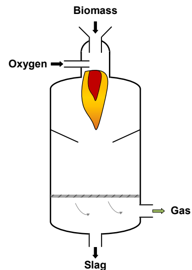
Principle of the entrained flow gasifier.
