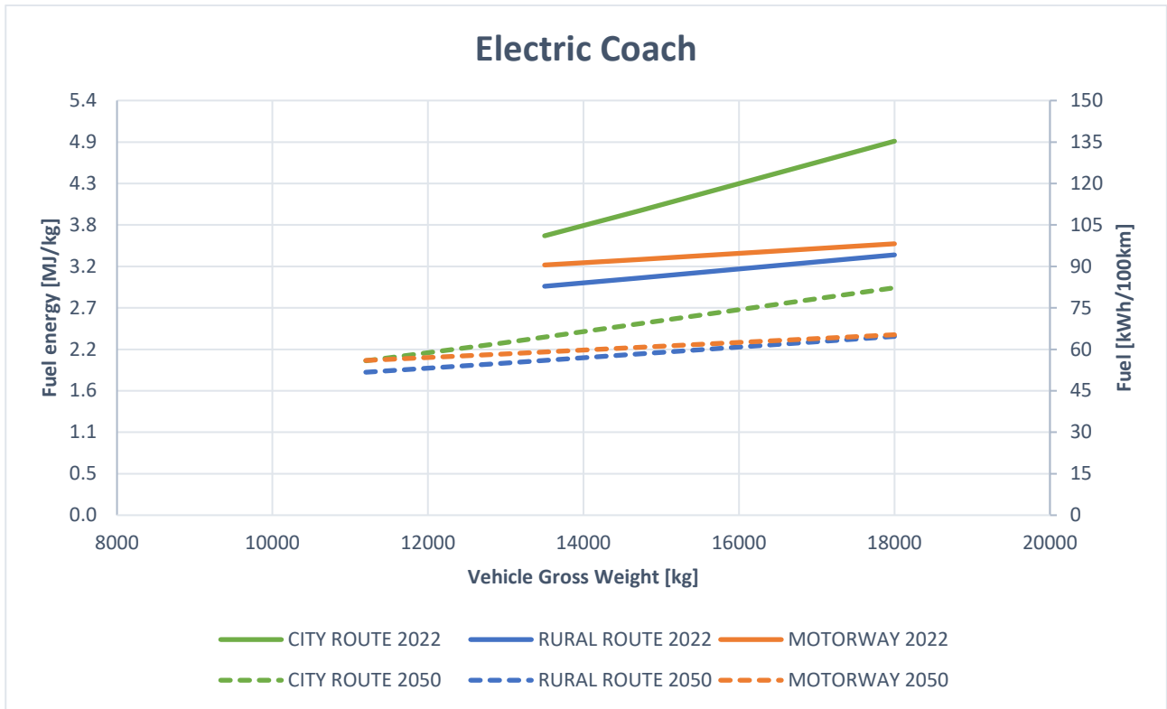
Figure 25 Predicted energy consumption of electric tourist buses.
