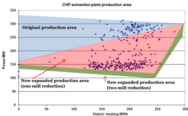
Figure 38: Change in production area due to investment in flexibility for a CHP extraction plant Before the changes, the minimum load was 45%, and the result of the changes (which took roughly half a year), was that the operation area was doubled, and the minimum load reduced to 36%. The dots in the figure represent each hour of production during the first month of production with the enhanced production area.
