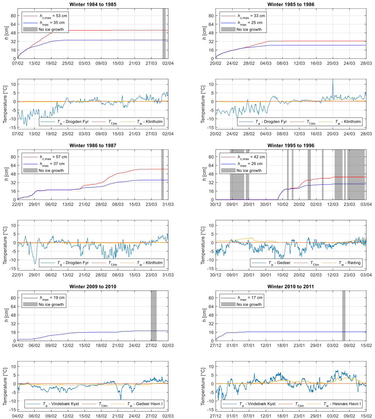
Figure C-2: Upper half of each pair of plots: Sheet ice thickness (dark blue curve), h , and consolidated layer thickness (red curve), h_c , as a function of time for winters 1984/1985 to 2010/2011. The bottom half of each pair of plots: The temperature curves shown in light blue are air temperatures, while the red lines are the freezing temperatures of the seawater at the site used in the modelling. SST temperatures are shown by the yellow curve.
