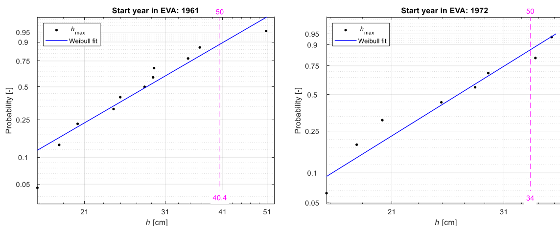
Figure 6-3: Probability of h_{\max} including a cumulative Weibull distribution fit. Please note that ice-free winters are not included. Left: The 50-year exceedance value of approximately 40 cm is indicated for the start year of 1961. Right: The 50-year exceedance value of approximately 34 cm is indicated for the start year of 1972.
