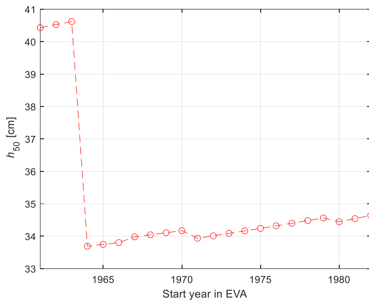
Figure 6-4: The 50-year sheet ice thickness, h_{50} as a function of the start year in the Extreme Value Analysis (EVA). The reason for the curve's slight upward slope is due to there being progressively fewer years used to assess the h_{50} -value. No EVA results are produced for start years after 1982 due to having too few data points to perform an EVA with sufficient quality.
