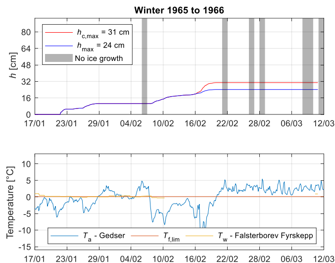
Figure 6-1: Example of thermal ice growth for the winter of 1965/1966. The grey areas are the selected days in which the ice will not grow due to the limiting number of days where ice can thermally grow.
