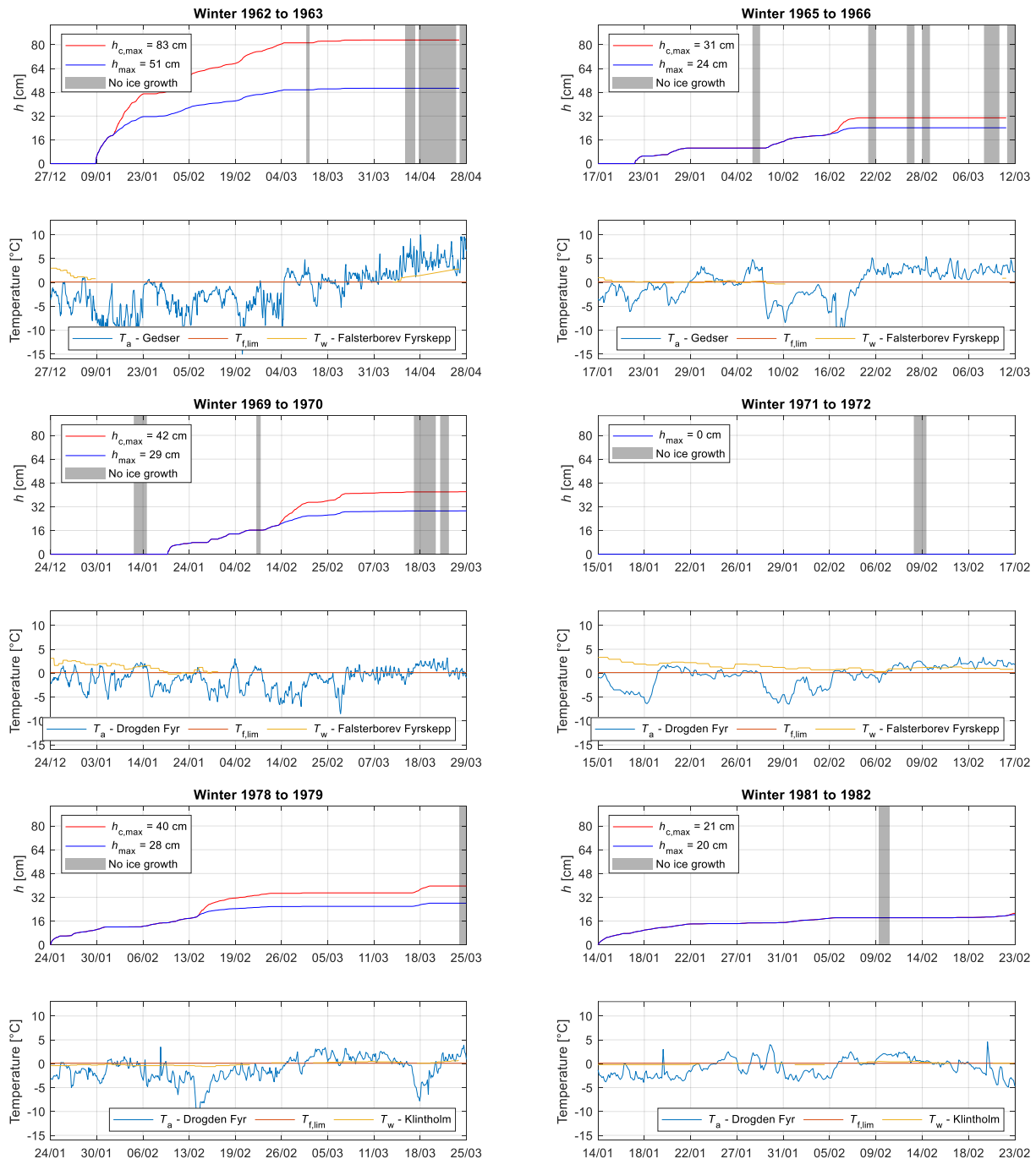
Figure C-1: Upper half of each pair of plots: Sheet ice thickness (dark blue curve), h , and consolidated layer thickness (red curve), h_c , as a function of time for winters 1962/1963 to 1981/1982. The bottom half of each pair of plots: The temperature curves shown in light blue are air temperatures, while the red lines are the freezing temperatures of the seawater at the site used in the modelling. SST temperatures are shown by the yellow curve.
