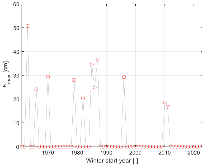
Figure 6-2: Maximum sheet ice thickness for each winter from 1960 to 2023 as a function of time (start year of the winter). The winters without any observations of sea ice are included as h_{\max} = 0 .
