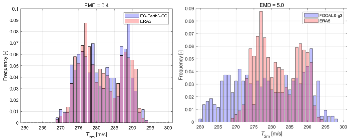
Figure 13-12: Example of climate models that passed (left) and failed (right) the EMD test of probability distribution similarity.
