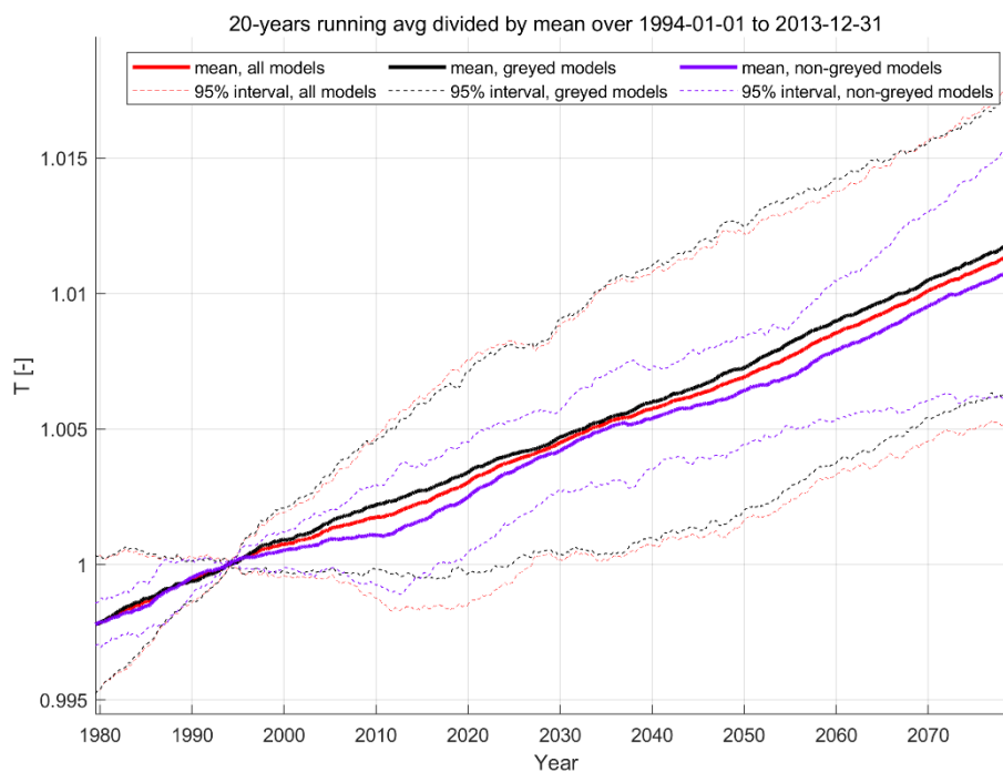
Figure 13-14: Example of model ensemble average and 95% confidence intervals for surface level air temperature in a 20-year running average relative to that of the period 1994-2014 (last 20 years of the climate model historical run). The red lines show the result that would be obtained when retaining all models, the black lines show the results only with the excluded models, and the purple lines show the results with the models retained after filtering.
