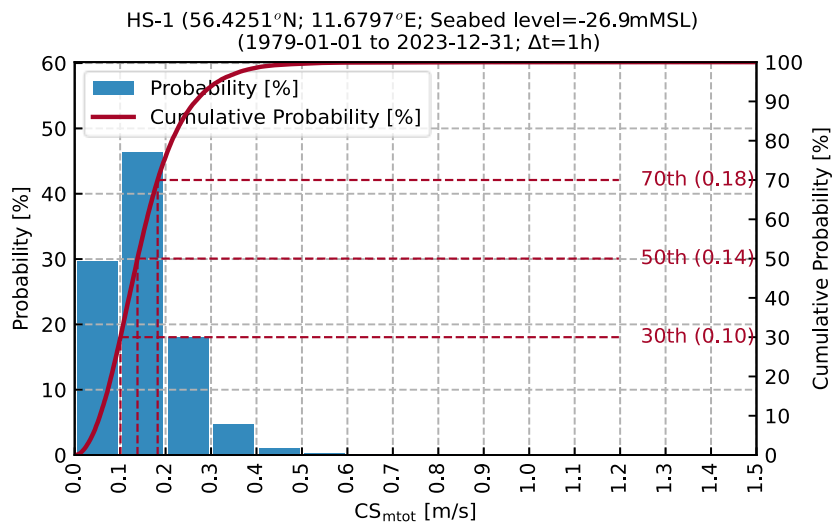
Figure 6-8 Probability plot of CS mt0t at HS-1.
