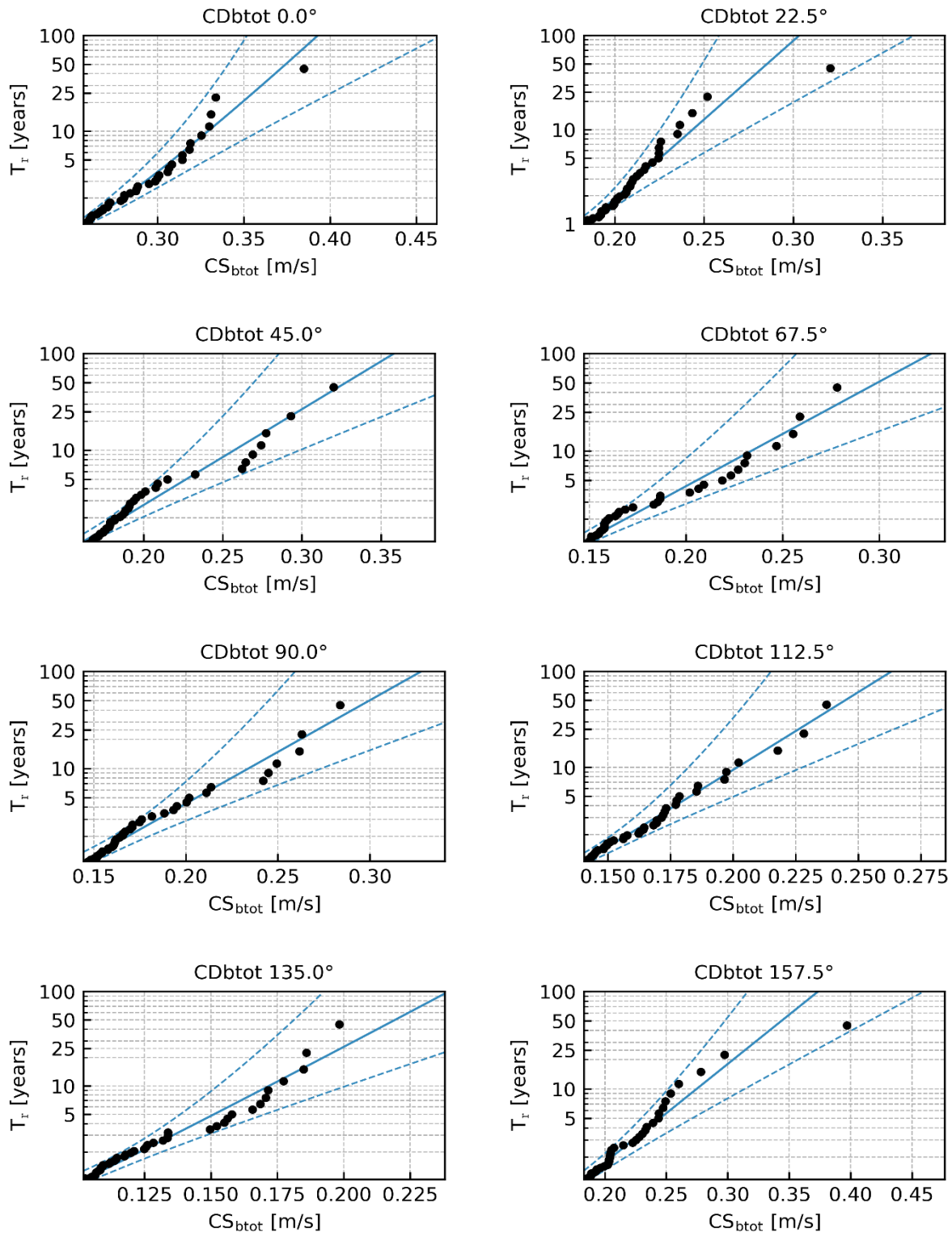
Figure 6-37 Marginal directional EVA estimates of CS_{btot} for CD_{btot} [ ^\circ N-going to] sectors every 22.5^\circ for HS-1. Weibull LS, \lambda = 1 . Confidence limits 2.5% -97.5%.
