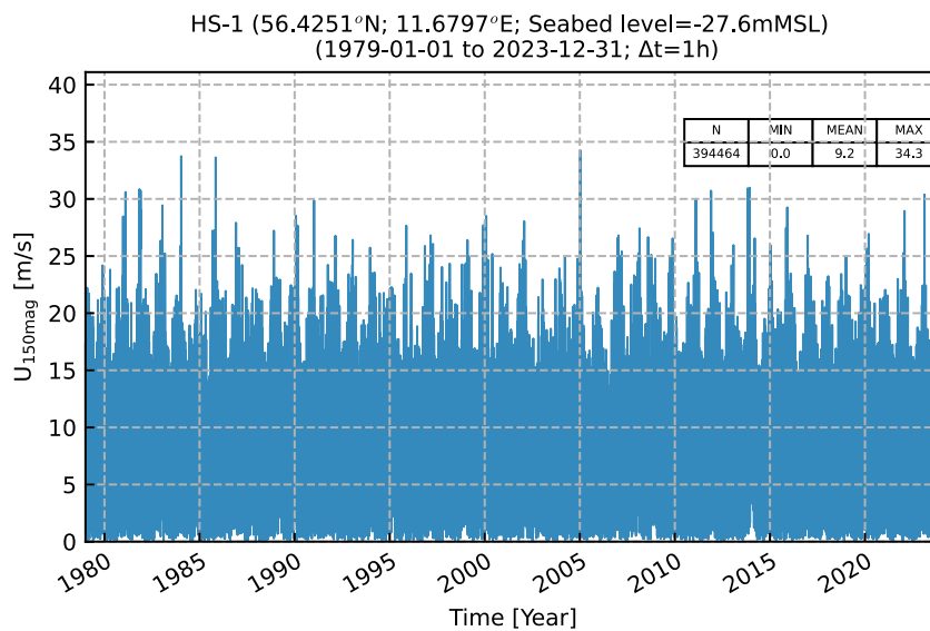
Figure 4-5 Time series of U_{150mag} at HS-1.
