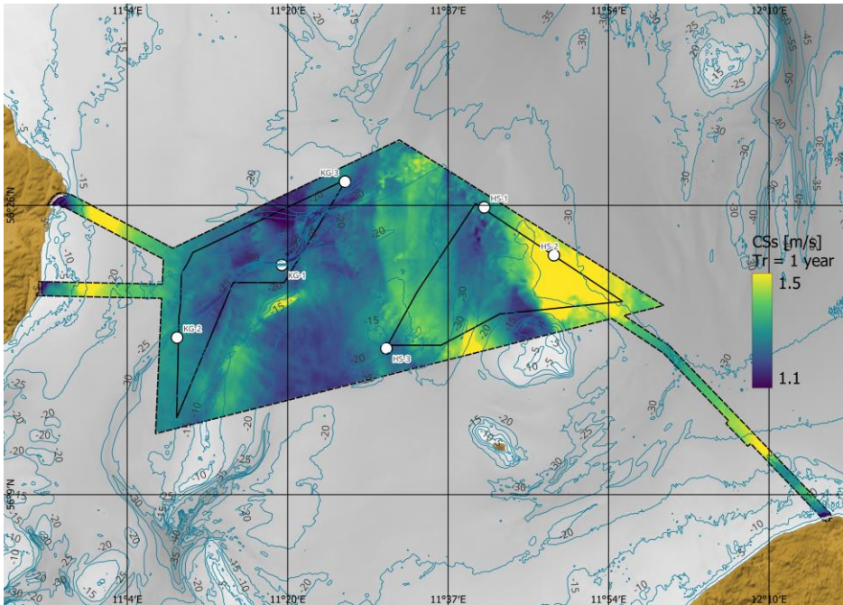
Figure 6-39 Spatial variation across the data delivery area of HS of CS_{\text{stot}} for return periods of 1 years. The colour map shows the current speed, and the contours show water depths.
