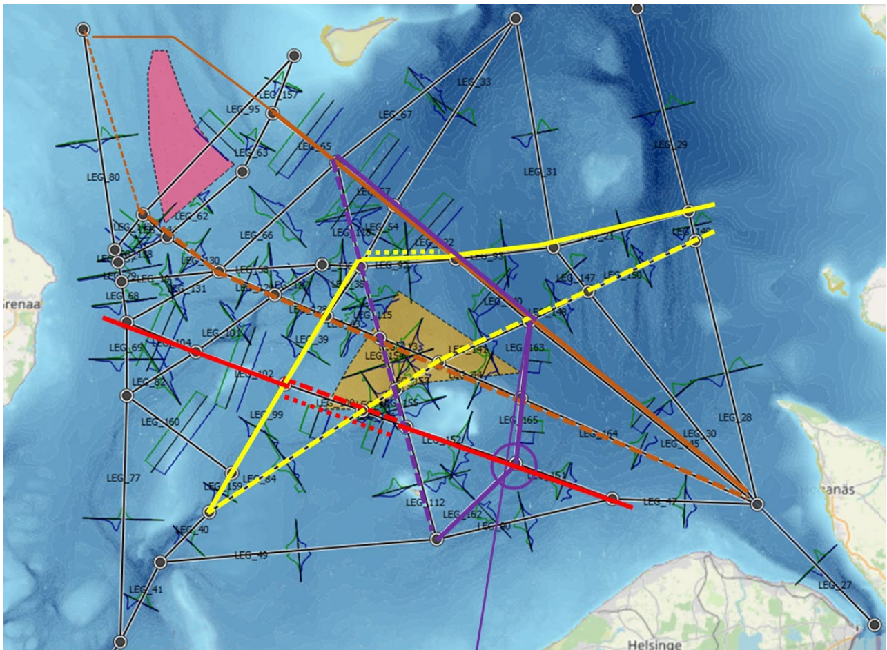
Figure 7 Construction phase. Broken lines represent the original (Base Case) routes, solid lines represent re-routing for the construction phase, dotted lines indicate legs where the lateral distributions have been adjusted to avoid the HES OWF, circles represent waypoints where bending incidents have been suppressed in the model
