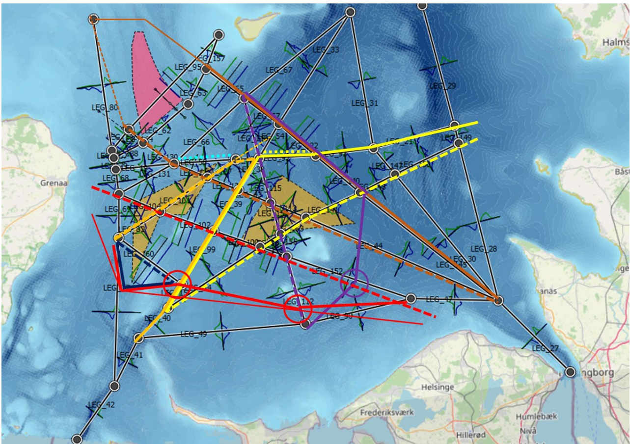
Figure 17. Cumulative changes in ship traffic for the operational phase of HES OWF and KA OWF. Broken lines represent the original (Base Case) routes, solid lines represent re-routing around the OWFs, dotted lines indicate legs where the lateral distributions have been adjusted to avoid the OWFs, circles represent waypoints where actual routes will be straight (as indicated by thin lines)
