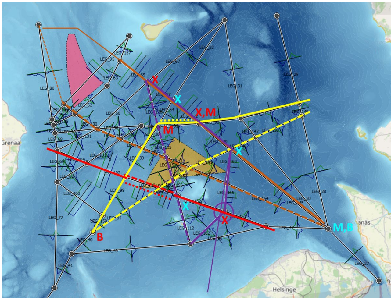
Figure 15 Assessment of changes in number of collisions at way point (crossing, merging, bending). Dashed lines indicate Base Case routes (existing traffic), drawn lines show re-routing around HES OWF. During Operational Phase fraction of original pleasure boats and fishing ships will use the existing routes (now
