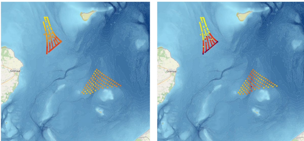
Figure 13 Operational Phase Scenario Allisions. Left: drifting allisions, right: powered allisions
