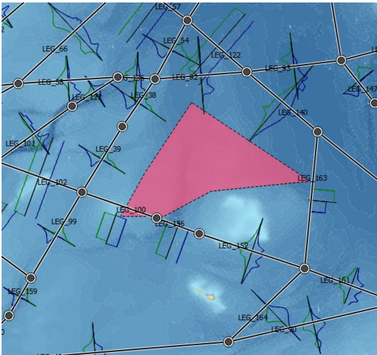
Figure 8 Adjustments of routes and lateral distributions around HES OWF during Construction Phase.
