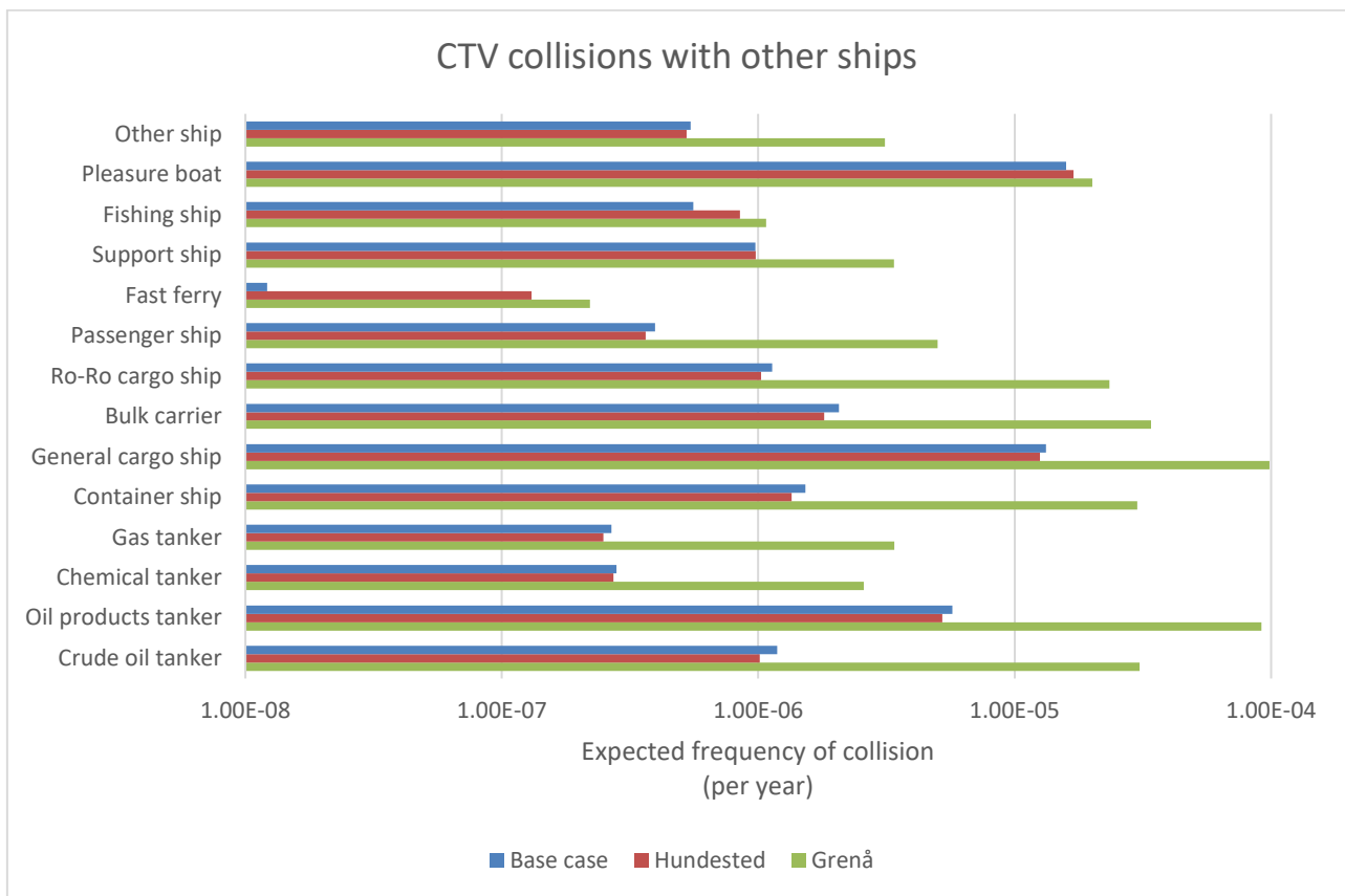
Figure 16 Change in number of collisions involving fast ferries/CTVs (striking or being struck) depending on whether CTVs servicing HES OWF operate from Hundested or Grenaa. All cases include CTVs servicing Anholt OWF from Grenaa. Collisions between two fast ferries are counted as one event.
