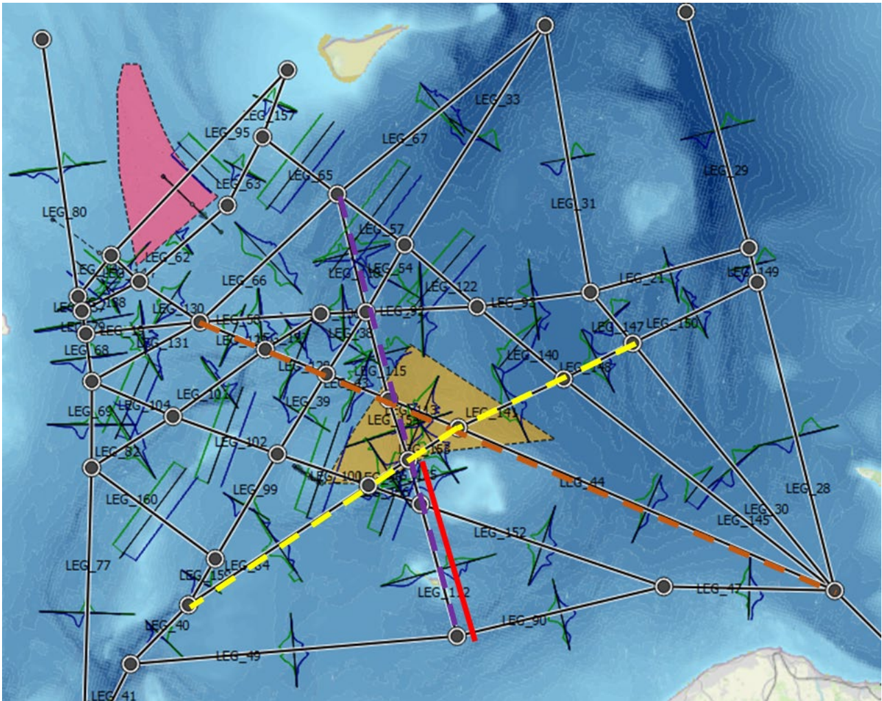
Figure 9 Operational phase. A fraction of the pleasure boats and fishing ships from the original routes (see also Figure 7), have been reinstated as per . Red line indicates CTVs servicing HES OWF from Hundested.
