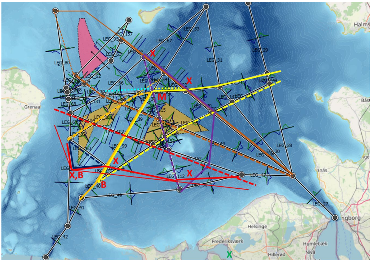
Figure 18 Assessment of changes in number of collisions at waypoints (crossing, merging, bending) for the cumulative case. Red letters point at waypoints where incidents are expected to increase, B=Bending incidents, M=Merging incidents, X=Crossing incidents.
