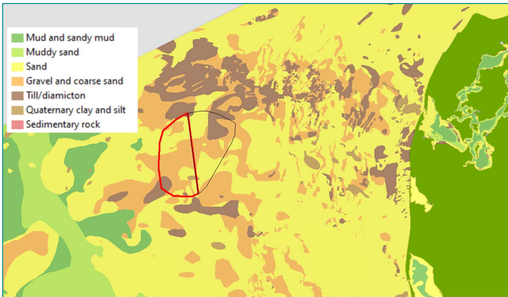
Figure 5-4. Geology, seabed surface (GEUS 2015). The red outline shows the general project development area for OWF – zone west. The adjacent OWF – zone east is highlighted with the black polygon.
