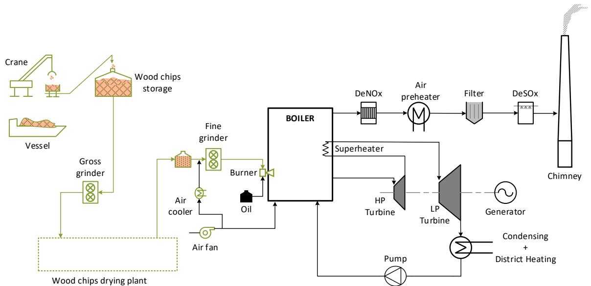
Figure 3: Sketch of a CHP plant converted to firing with wood chips with its existing boiler. The green elements indicate the equipment that needs to be added, replaced or refurbished.
