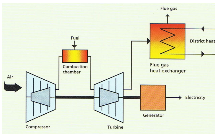
Figure 1 Diagram of a simple cycle plant designed for combined heat and power production.
