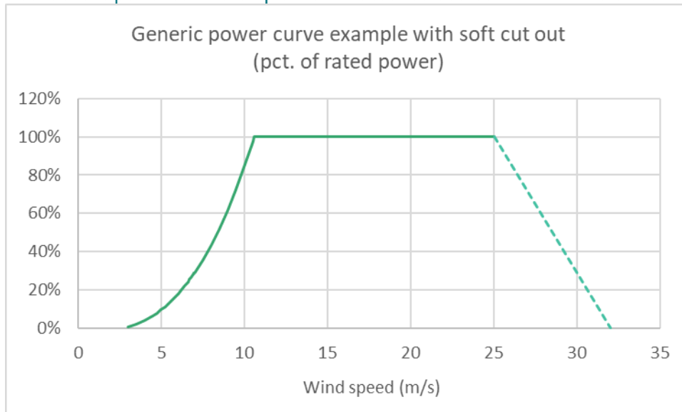
Figure 36: Generic power curve example with soft cut out. Source: IEA 15MW reference turbine.
