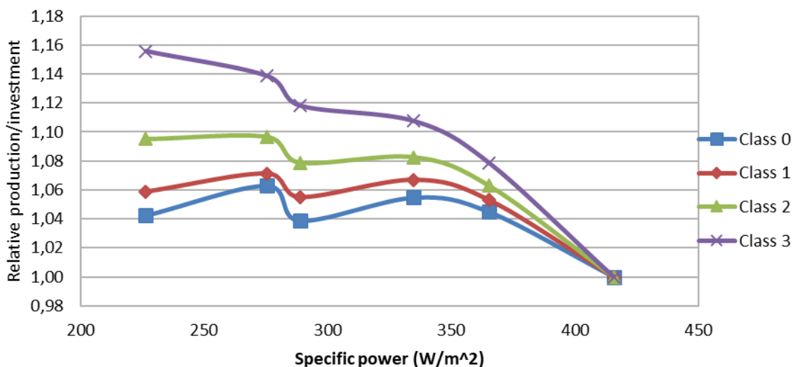
Figure 25 The production relative to the investment cost based on current available Vestas turbines for different rotor areas, generator size is 3.6 - 4 MW for all (= different specific power).
