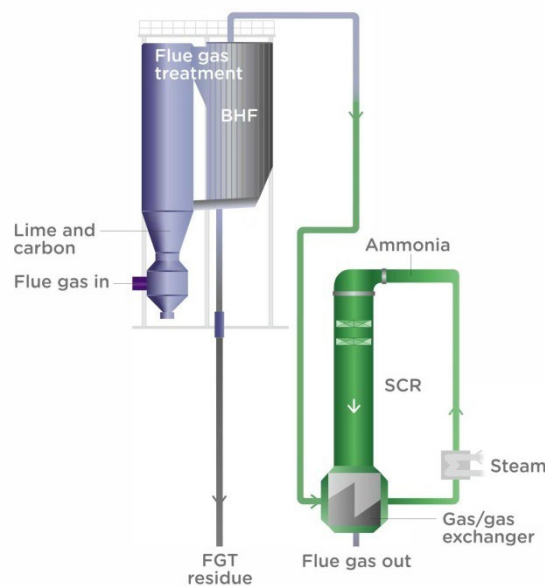
Figure 6 Flue gas treatment system (dry/semi-dry) including reactor with injection of hydrated lime, a bag house filter and an SCR system with gas/gas heat exchanger, steam reheat, ammonia injection and catalyst.
