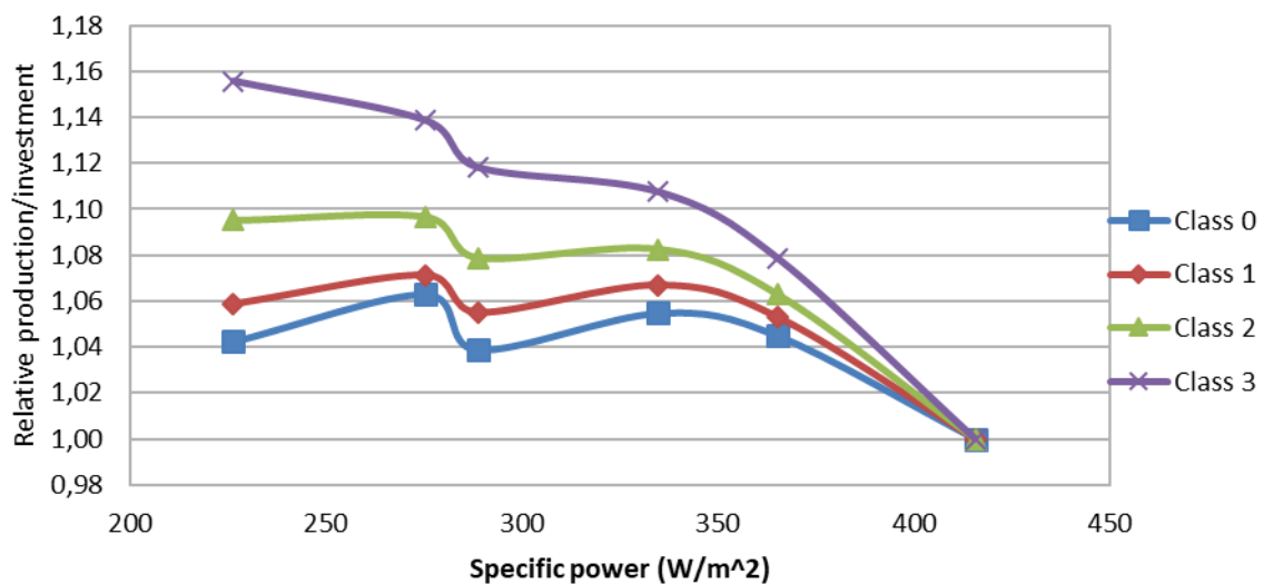
Figure 25 The production relative to the investment cost based on current available Vestas turbines for different rotor areas, generator size is 3.6 - 4 MW for all (= different specific power).
