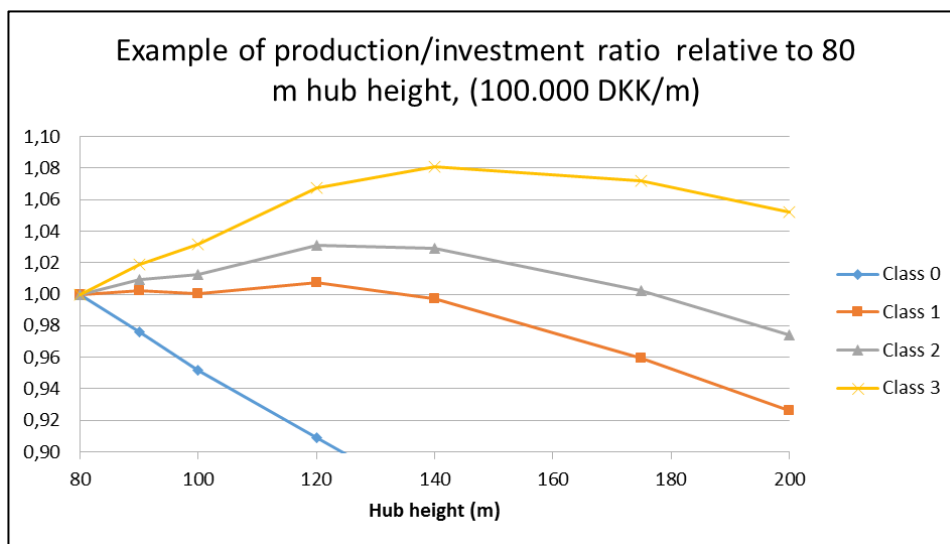
Figure 23 The production increase relative to the investment cost based on current available Vestas turbines. By increasing height, costs are extrapolated using DKK 100.000 per m hub height increase; the rotor area is kept constant.
