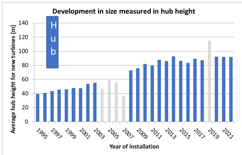
Figure 19 Average hub height for new turbines (rated power > 25 kW) [2]
