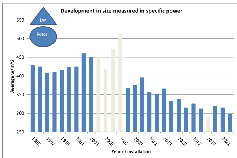
Figure 21 Average specific power for new turbines (rated power > 25 kW) [2]
