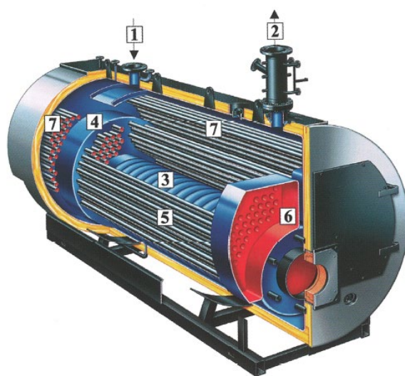
Figure 1 Typical flue gas tube boiler for the power range 1- 20 MW. Combustion takes place in the firetube (3). Flue gasses then passes inside a number of flue gas tubes ((5) & (7)) transmitting further heat to the boiler water around these. The water connections (forward/return) are on the top ((2) & (1)) [6].
