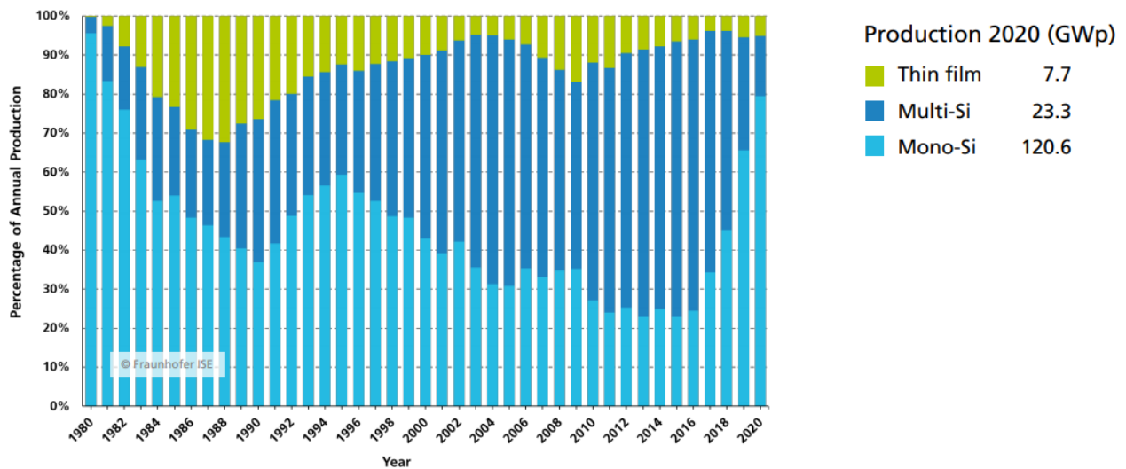
Figure 1 Historical market shares of different cell technologies (Ref. 9).
