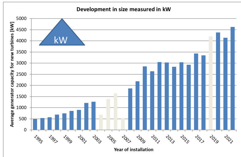
Figure 17 Average generator capacity for new turbines (rated power > 25 kW) [2]
