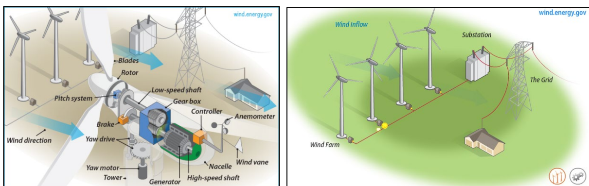
Figure 11 General turbine technology and electrical system.
