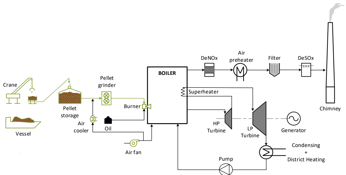
Figure 1: Sketch of a CHP plant converted to firing with wood pellets. The green elements indicate the equipment that needs to be added, replaced or refurbished.
