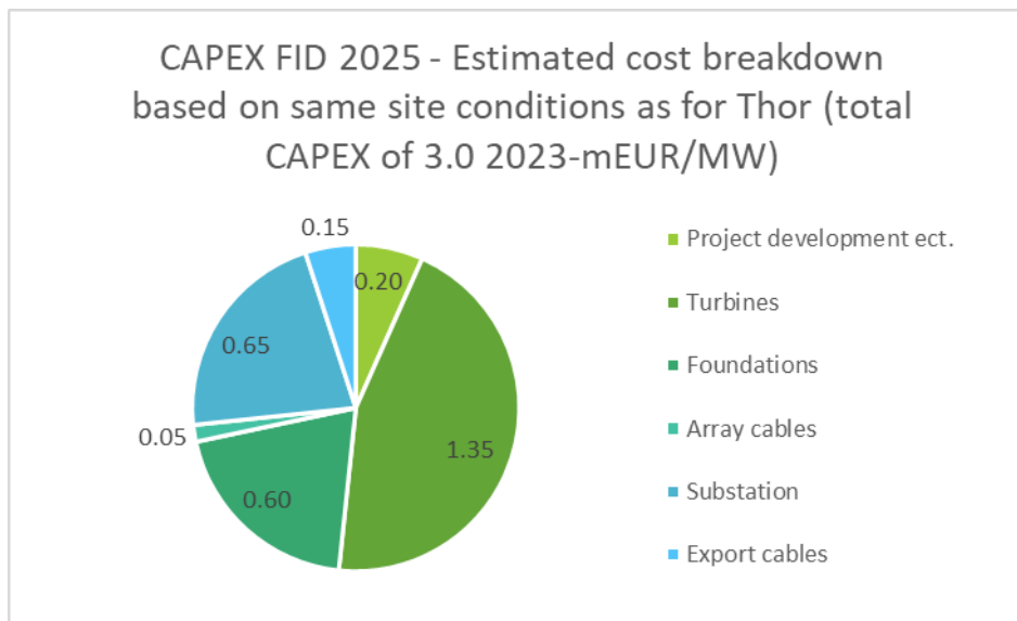
Figure 43: Estimated cost breakdown for a project like Thor taking FID in 2025.
