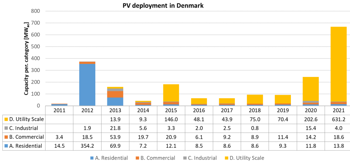
Figure 10 Installed capacity (MW ac /year) in Denmark. Based on data from the Danish Energy Agency (Stamdataregister) processed into the following categories: Residential <10, Commercial <250, Industrial <1000 and Utility scale >1000 kW. Data processed by categorizing and addition of known grid-connected projects that had not been registered in the Stamdataregister
