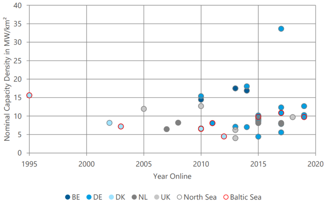
Figure 38: Nominal capacity densities of European offshore wind farms [4]
