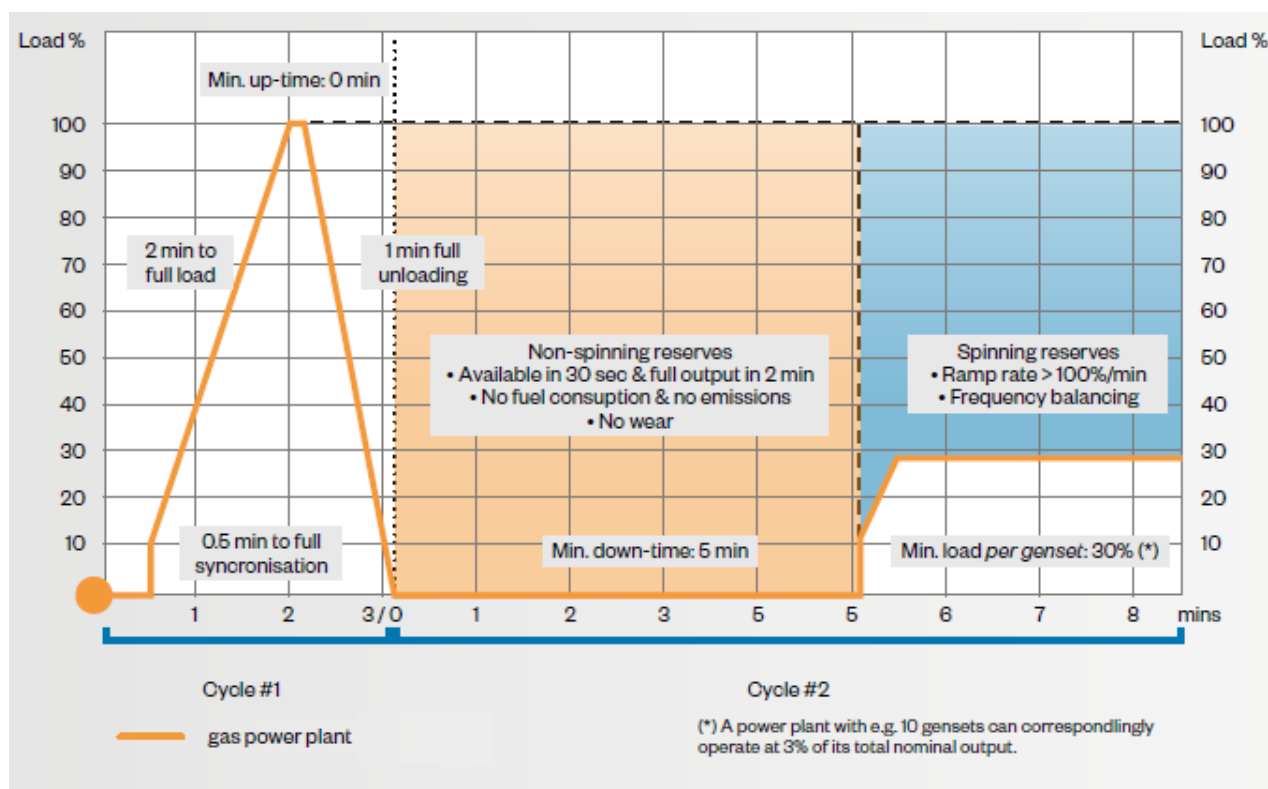
Figure 2 Dynamic characteristic of a gas engine power plant [13].
