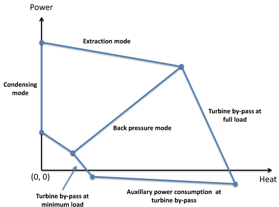
Figure 5 Generic PQ-diagram for extraction CHP
