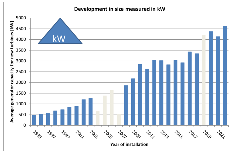
Figure 17 Average generator capacity for new turbines (rated power > 25 kW) [2]
