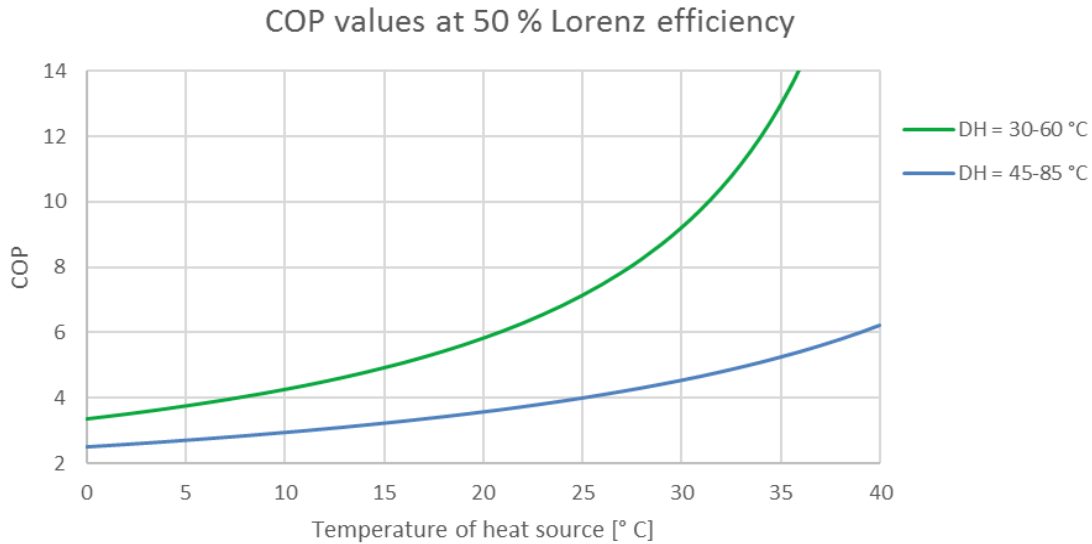
Figure 3 Attainable COP values of a compression heat pump with varying heat source temperatures at two different sink requirements.
