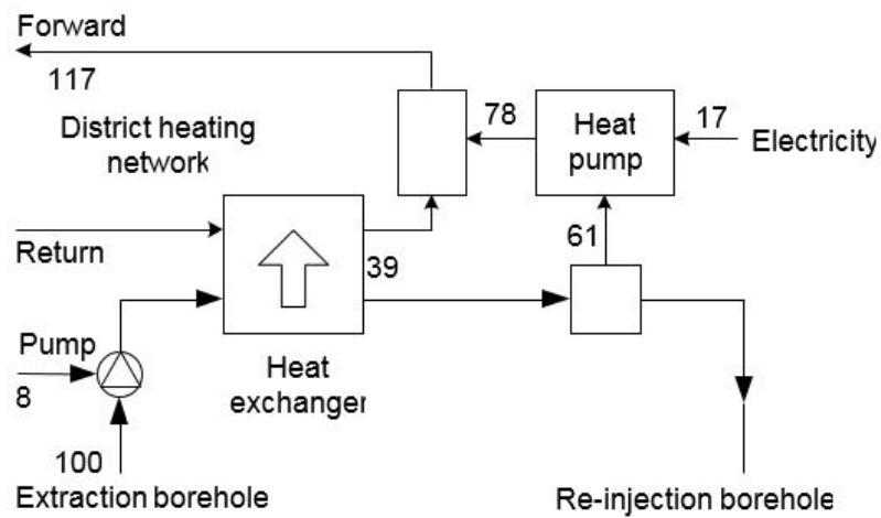
Figure 0-5: Example of a system with an electric heat pump. The COP of the electric heat pump is approximately 4.6 and the total efficiency (COP) of the system is approximately 4.7.
