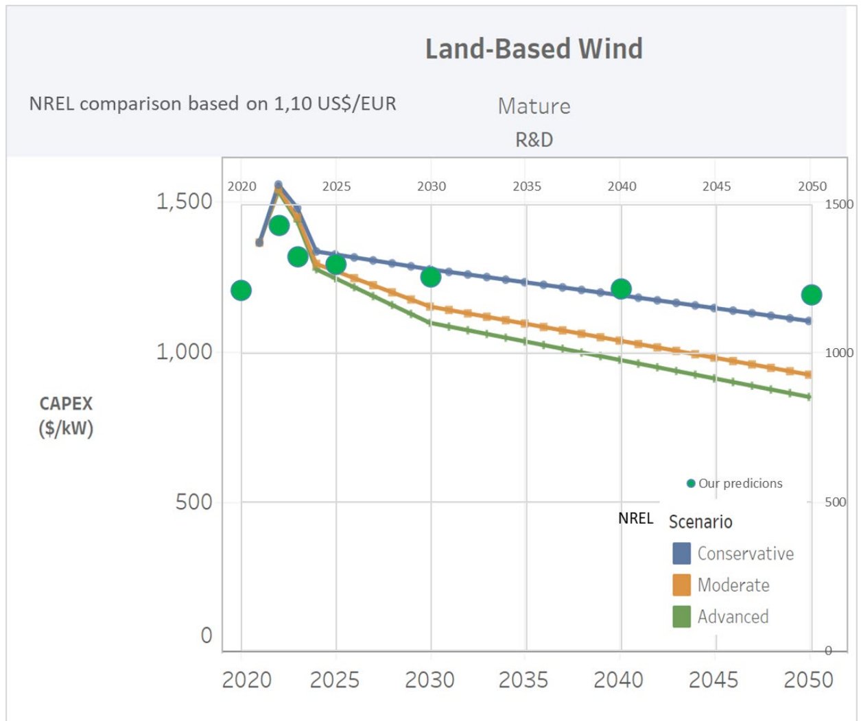
Figure 31 The resulting CAPEX (2020 prices) for onshore wind projects put on top of NREL similar prediction scenarios.
