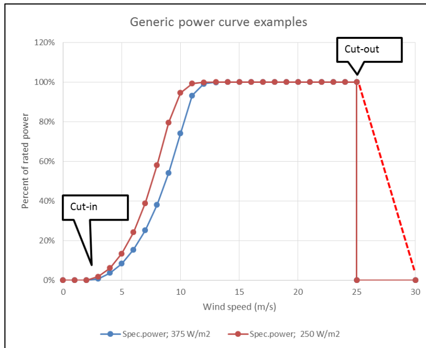
Figure 12 Turbine power curves (Information's from expert workshop held by DEA 27-4-2015). Specific power values refer to e.g. 3 MW with 124m rotor diameter (250 W/m 2 ) and 3 MW with 101 m rotor diameter (375 W/m 2 )
