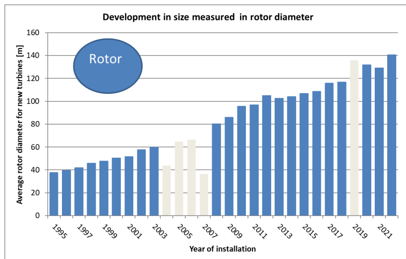
Figure 18 Average rotor diameter for new turbines (rated power > 25 kW) [2]
