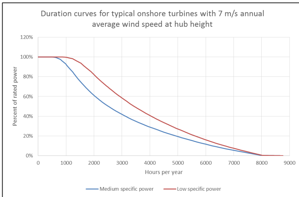
Figure 13 Duration curve for typical modern onshore wind turbines (> 2 MW) located in Denmark (DTU International Energy Report - Wind Energy, 2014). The two curves are based on the V117 3.3 MW (307 W/m 2 ) and V126 3.3 MW (265 W/m 2 ) wind turbines.
