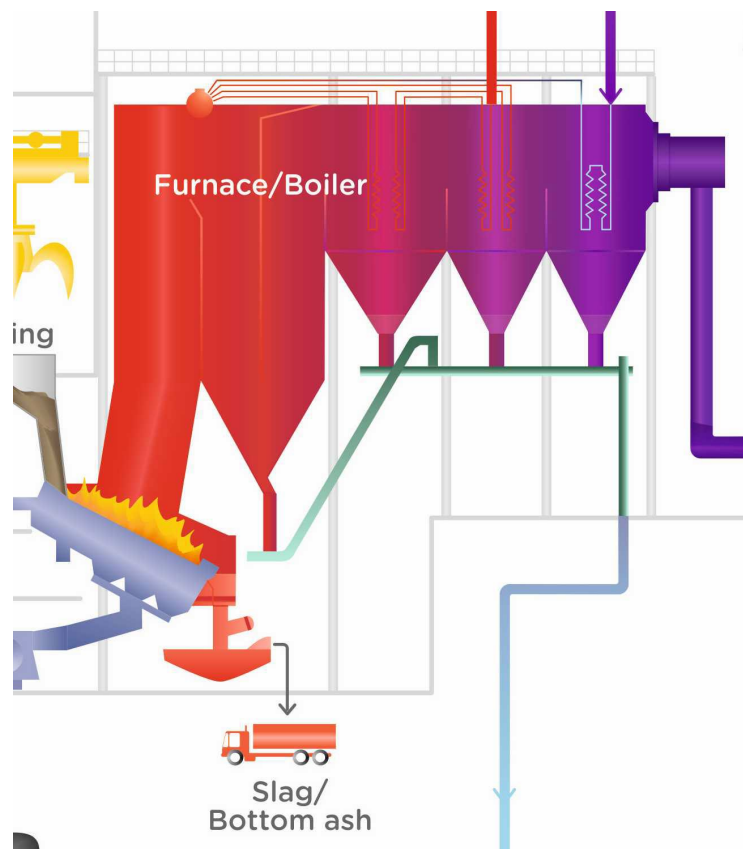
Figure 2 Furnace/boiler system
