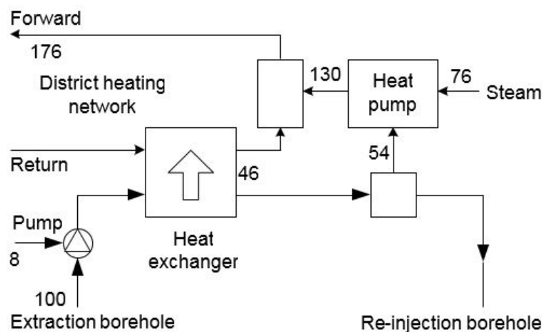
Figure 0-4: Example of a geothermal system with an absorption heat pump. The numbers indicate the energy flows relative to the extracted amount of geothermal heat from the reservoir, which is set at 100 energy units. The heat pump COP is 1.7 and the total efficiency of the system is approximately 2.1.
