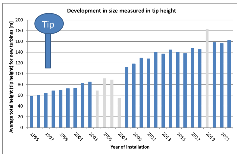
Figure 20 Average tip height for new turbines (rated power > 25 kW) [2]
