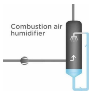
Figure 8 Combustion air humidifier, where water heated by a low-temperature source is evaporated into the combustion air flow.
