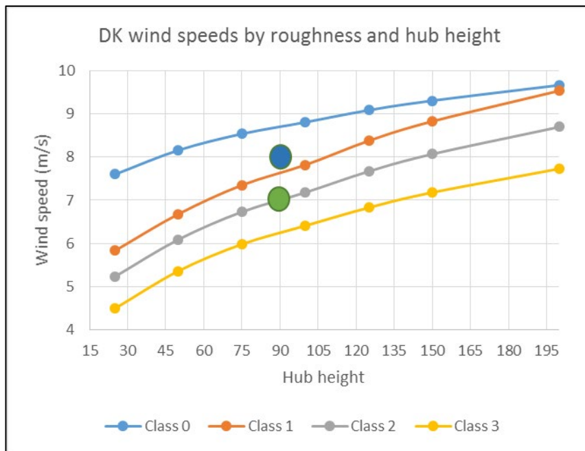
Figure 14 Annual average wind speeds as a function of hub height and roughness class for flat terrain. The green dot represents a typical modern inland site; the blue dot represents a typical coastal site. The typical hub height is 90 m.
