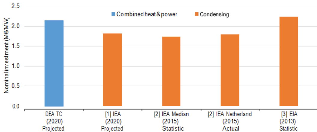
Figure 2: Nominal investment in coal fired power plants (2015M€/MW). The years in () indicate the year of the commission or statistic.
