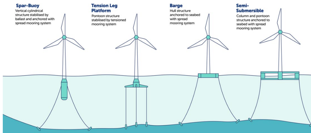
Figure 35: Floating foundation structures – dominant types [13], [14]
