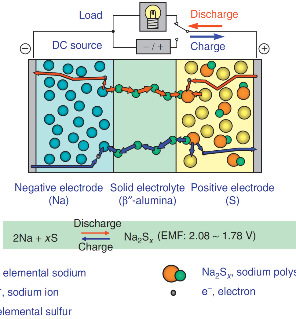
Figure 2: Graphical schematic of the reaction process and the full cell reaction. EMF: electromotive force. [4]
