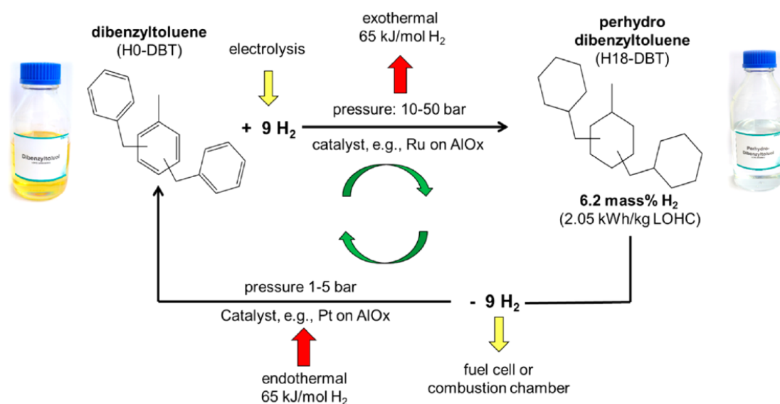
Figure 22: Hydrogen storage using DBT-LOHC system[50]
