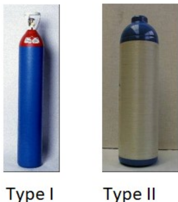
Figure 17: (left) Type I steel cylinder, (right) Type II steel cylinder with composite wrap [23]
