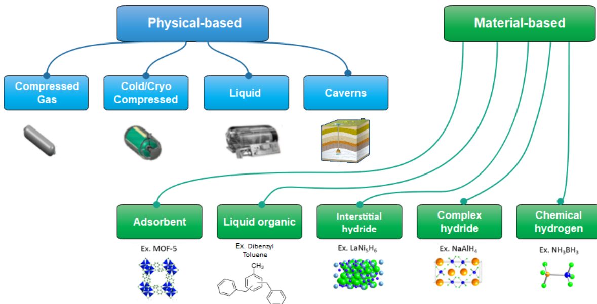
Figure 14: Hydrogen storage categories (icons from [6])
