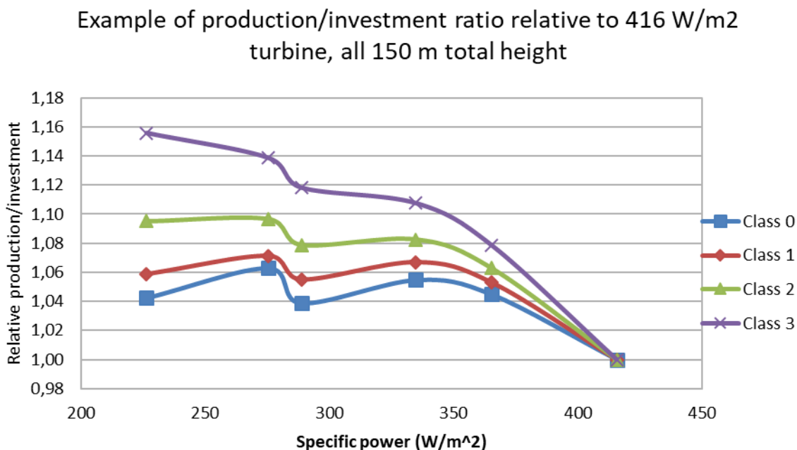
Figure 25 The production relative to the investment cost based on current available Vestas turbines for different rotor areas, generator size is 3.6 - 4 MW for all (= different specific power).
