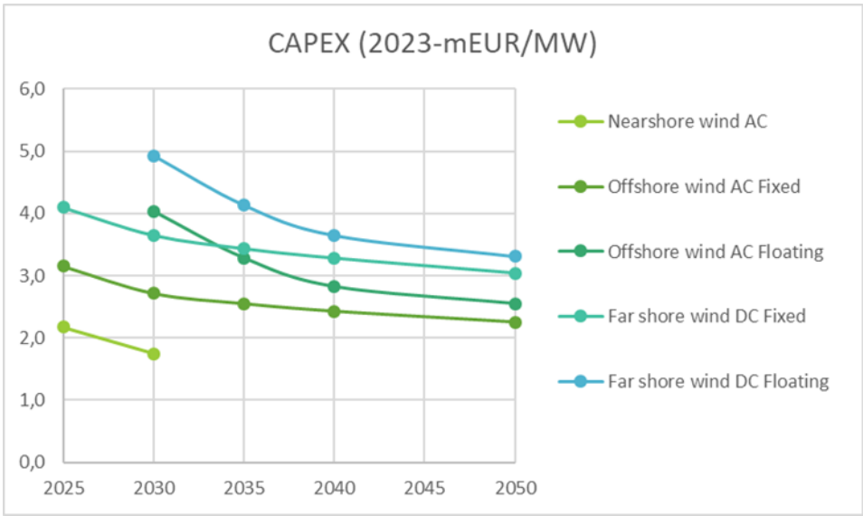
Figure 44: CAPEX projections (2023-mEUR/MW) (updated in May 2025 after a correction).
