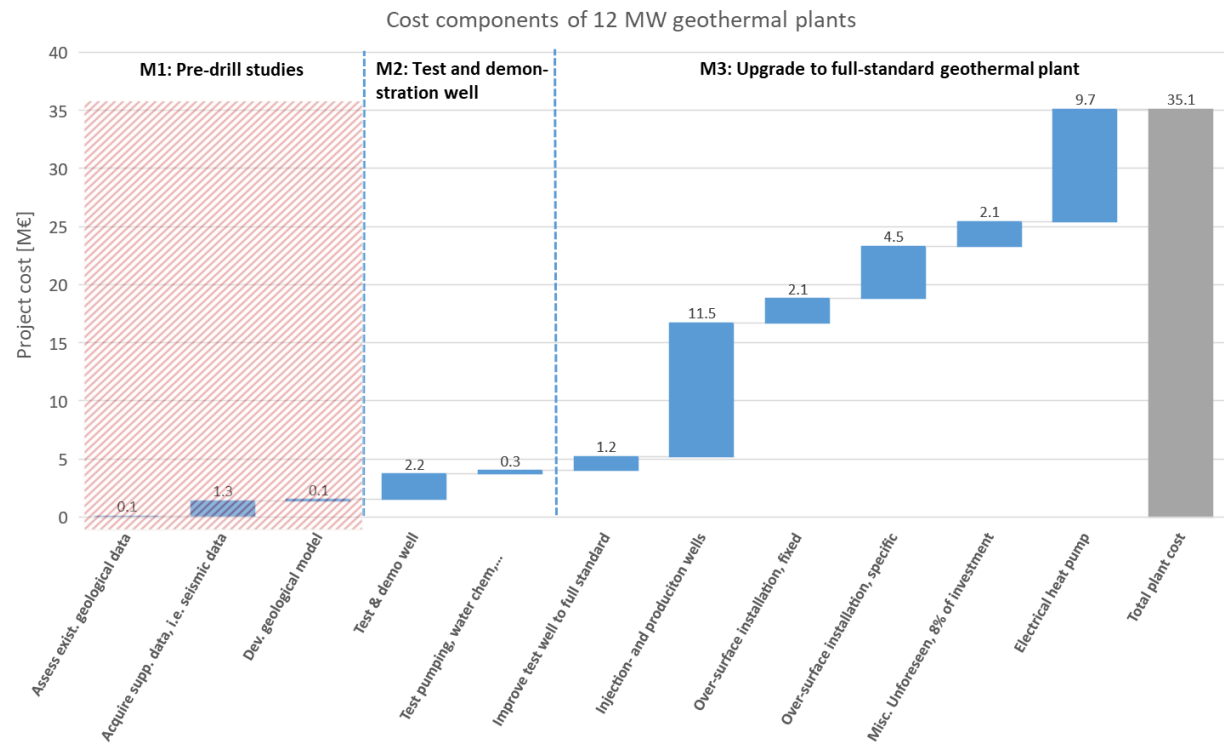
Figure 0-11 Cost components of a 12 MW geothermal plant 1.a - 1,200 m reservoir with electrical heat pump. Definition of milestones (M1-3) is given in [14].
