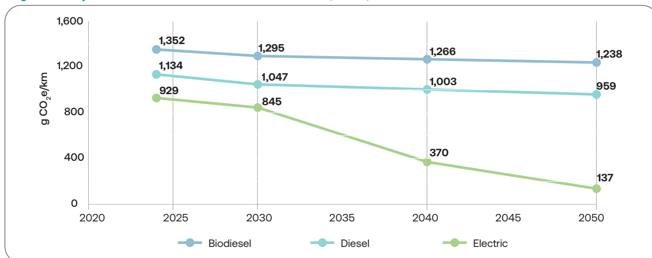
Figure 12. Projection of WTW GHG emissions of B35 biodiesel, diesel, and electric bus models until 2050
