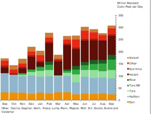
Gas Production
