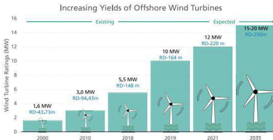
Figure 33. Increasing yield of offshore wind turbines [9].
