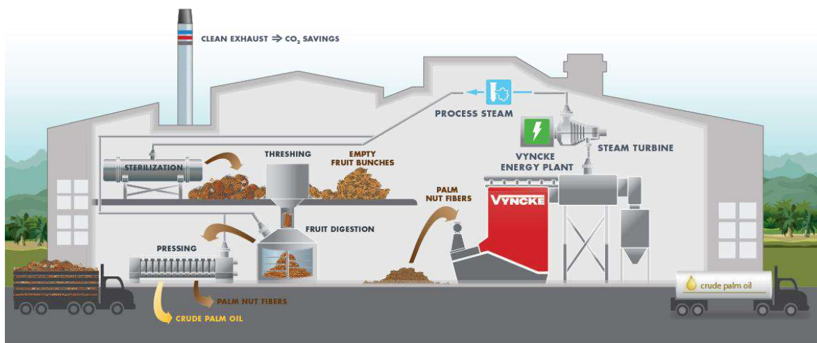
Figure 64. Typical combined heat and power from palm oil solid waste [8].
