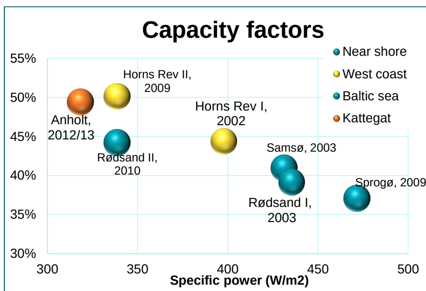
Figure 35. Capacity Factor shown as function of the Specific Power ( W/m^2 ) for Danish Offshore wind turbine projects. The three projects most left are the latest ones among the sample. (Figure from a previous version of Technology Catalogue [28]).
