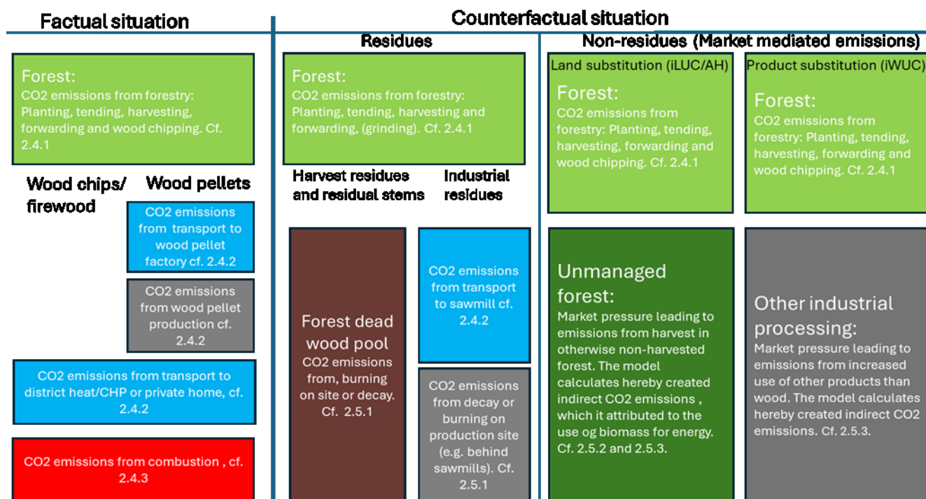
Figure 1. Overview of the model framework. The model calculates the sum of all emissions in the factual situation, deducts emissions from the residual counterfactual and adds market mediated emissions from non-residues.
