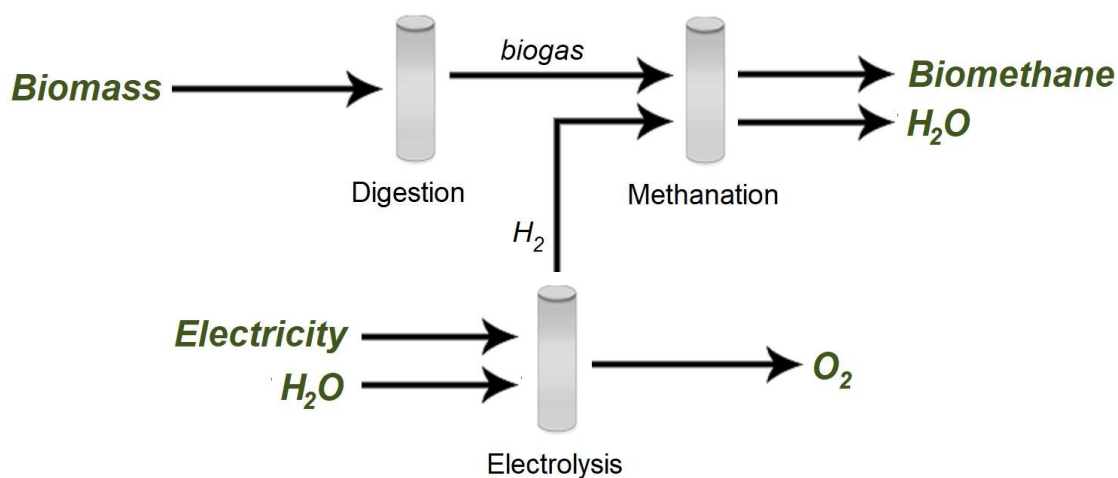
Figure 1 SNG Process
