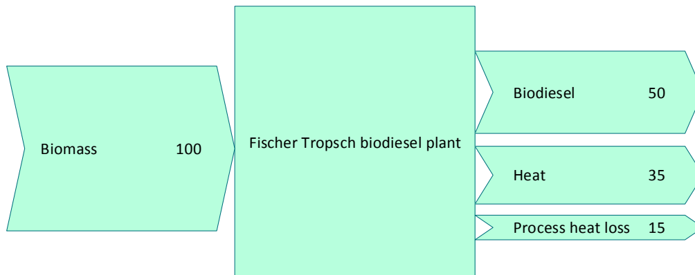
Sankey diagram of gasifier based Fischer-Tropsch plant in 2030.
