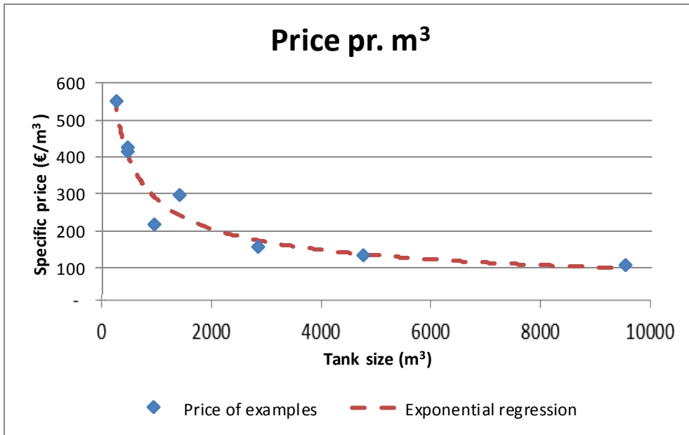
Figure 3: Specific price pr. m 3 by total size of tank, incl. foundation [2 & 4].
