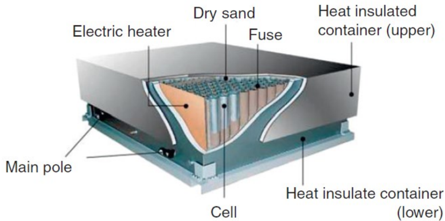
Figure 3: Illustration of Na-S battery module. [4]
