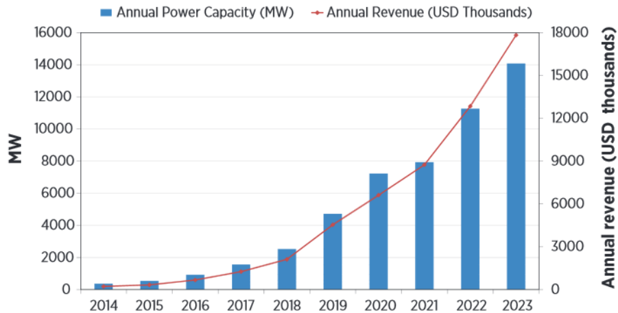
Figure 10: Worldwide forecast of battery storage capacity (MW) and annual revenue (USD) for utility-scale applications [48].
