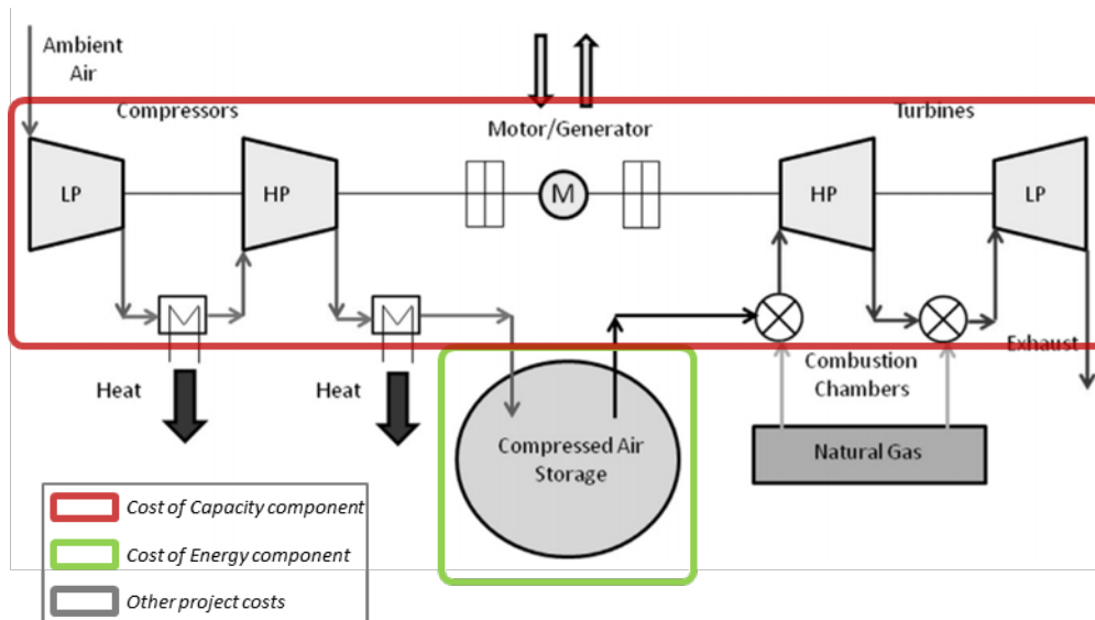
Figure 7 Components and their categorization for CAES. Source: elaboration of [5].
