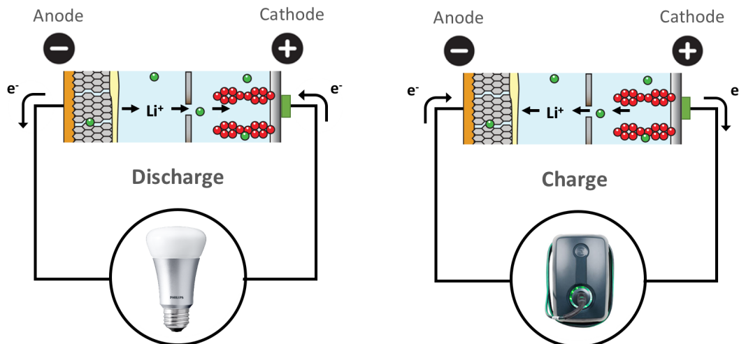
Figure 2. Schematic diagram of a LIB system in charge and discharge mode. During discharge the green \text{Li}^+ ions moves from the negative electrode (left side) to the positive electrode. The process is reversed during charge mode (right side).
