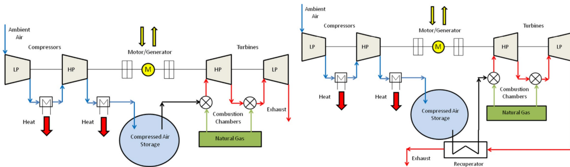
Figure 1: Operating principle of the CAES plant Huntorf (left) and the McIntosh (right) [1]
