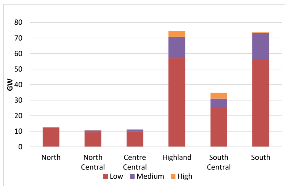
Figure 24: Resource potentials for onshore wind generation capacity per region and wind speed class implemented in the Balmorel model. Low: 4.5-5.5 m/s, Medium: 5.5-6 m/s, High: over 6 m/s (all at 80 m height).
