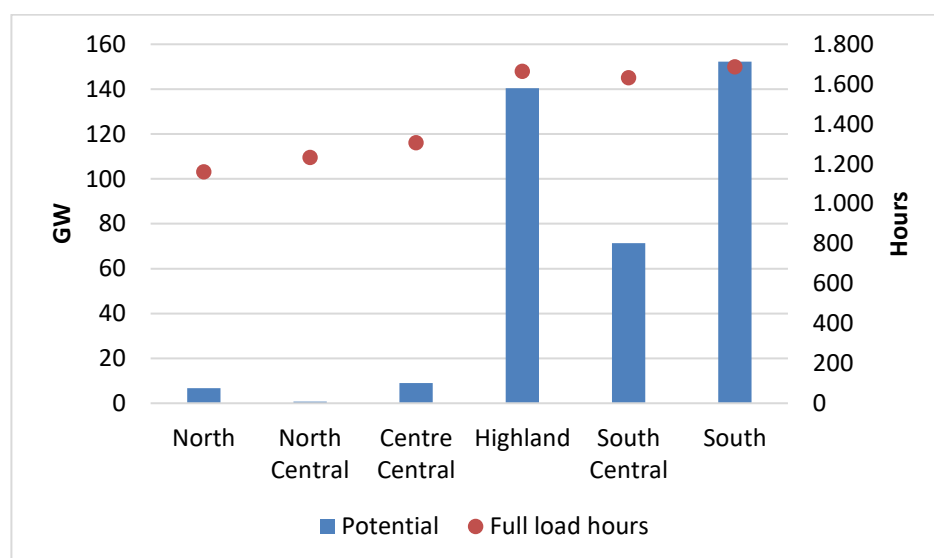
Figure 26: Solar potential and full load hours per region implemented in Balmore.
