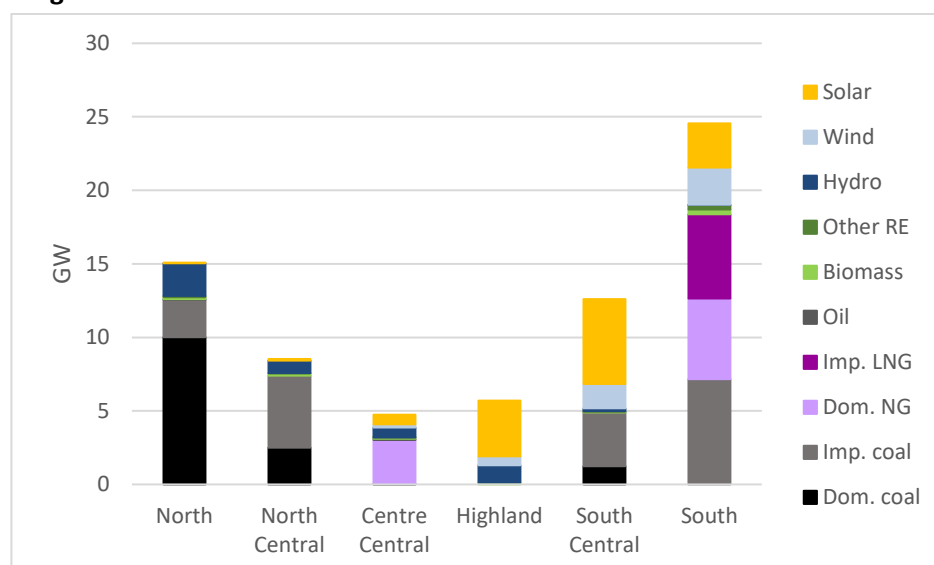
Figure 4: Existing and committed capacity per region (by 2025)
