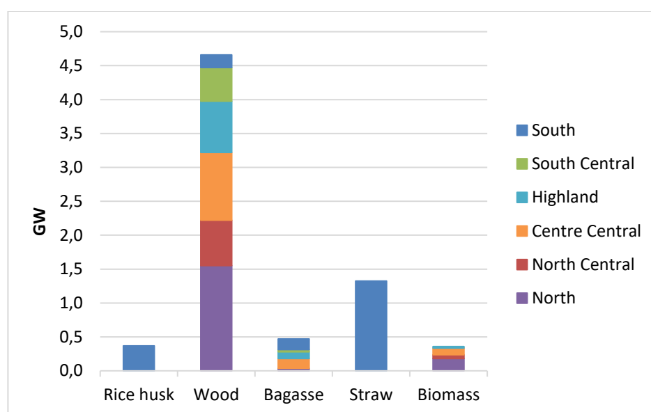
Figure 20: Resource limits on biomass-fired power generation capacity implemented in the Balmorel model (GW).
