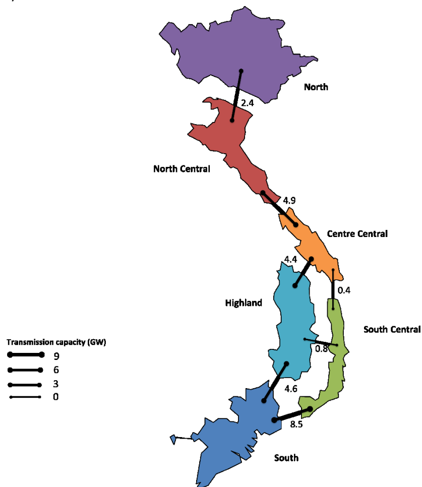
Figure 1. Current interconnectors in Vietnam (2019).
