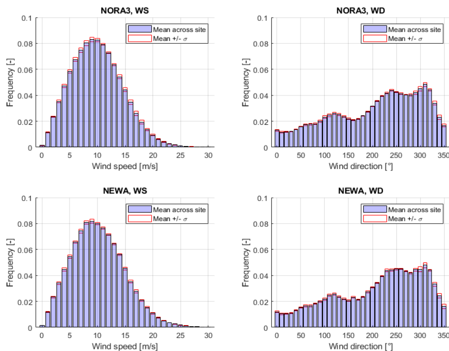
Figure 5-3: Wind speed (left) and wind direction (right) distributions for the different NORA3 (top) and NEWA (bottom). The blue bars show the mean frequency at each wind speed- and direction bin, while the red bars show the mean +/- 1 standard deviation.
