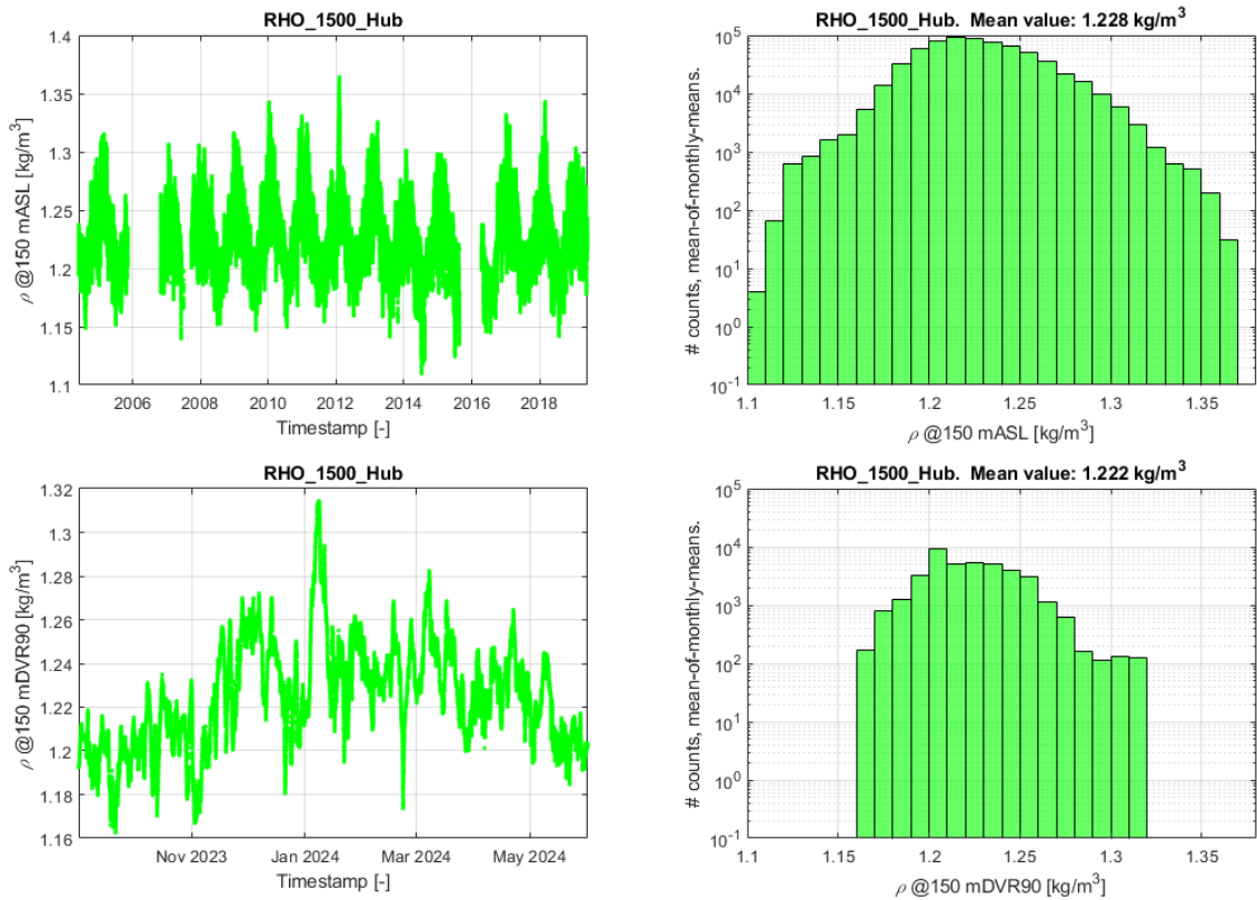
Figure 6-17: Air density at 150 mASL from the Høvsøre measurements (top) and 150 mDVR90 from the NSI-LB-3 measurements (bottom). The left part of the figure shows the model time series, and the right part of the figure shows an MoMM histogram of the values with a logarithmic 2 nd axis. The MoMM mean value is shown in the title above the histogram.
