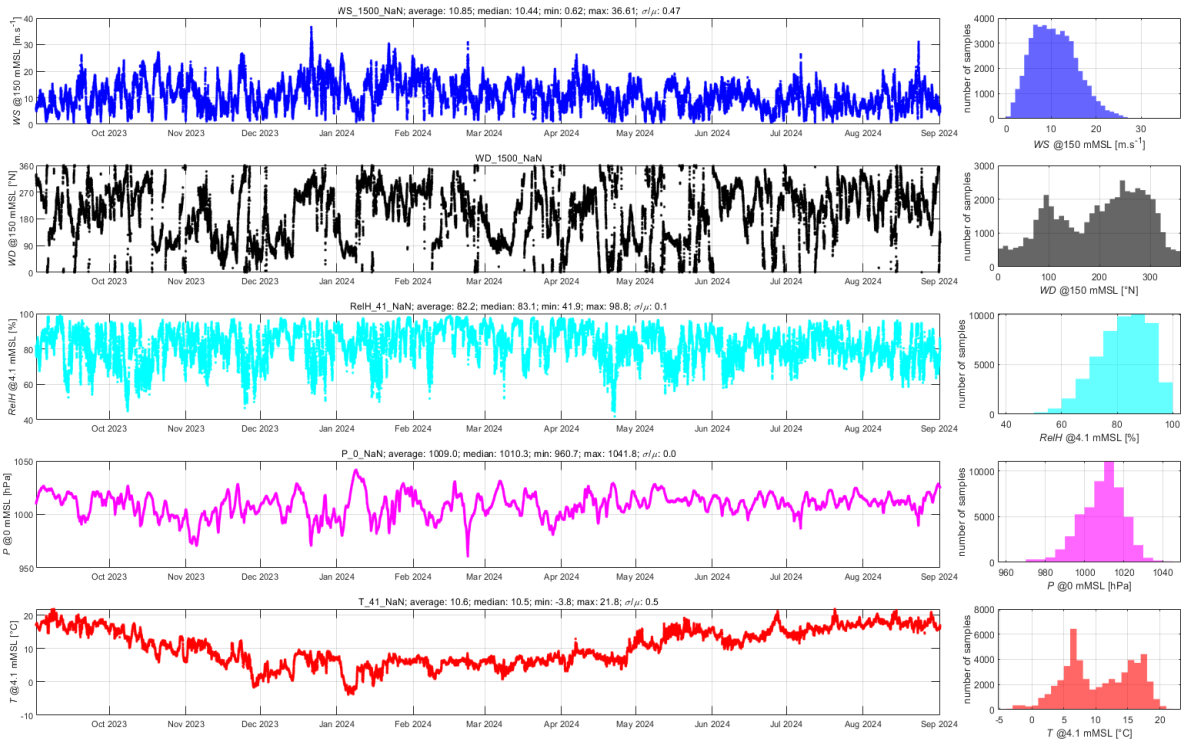
Figure B-4: Time series of wind speed and wind direction at 150 mMSL, as well as surface level air temperature, relative humidity and air pressure collected at NSI-3-LB.
