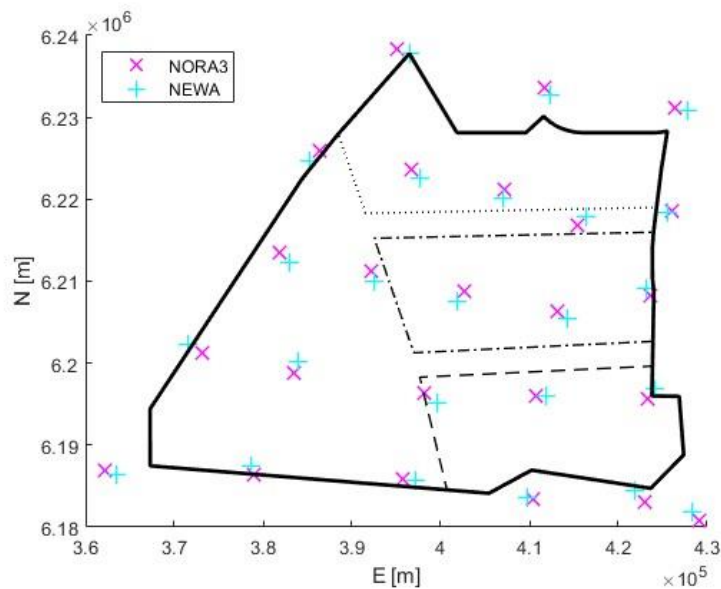
Figure 5-1: Locations of the NORA3 (magenta) and NEWA (light blue) nodes used for the analyses in this section. CRS: WGS84 / UTM Zone 32N.
