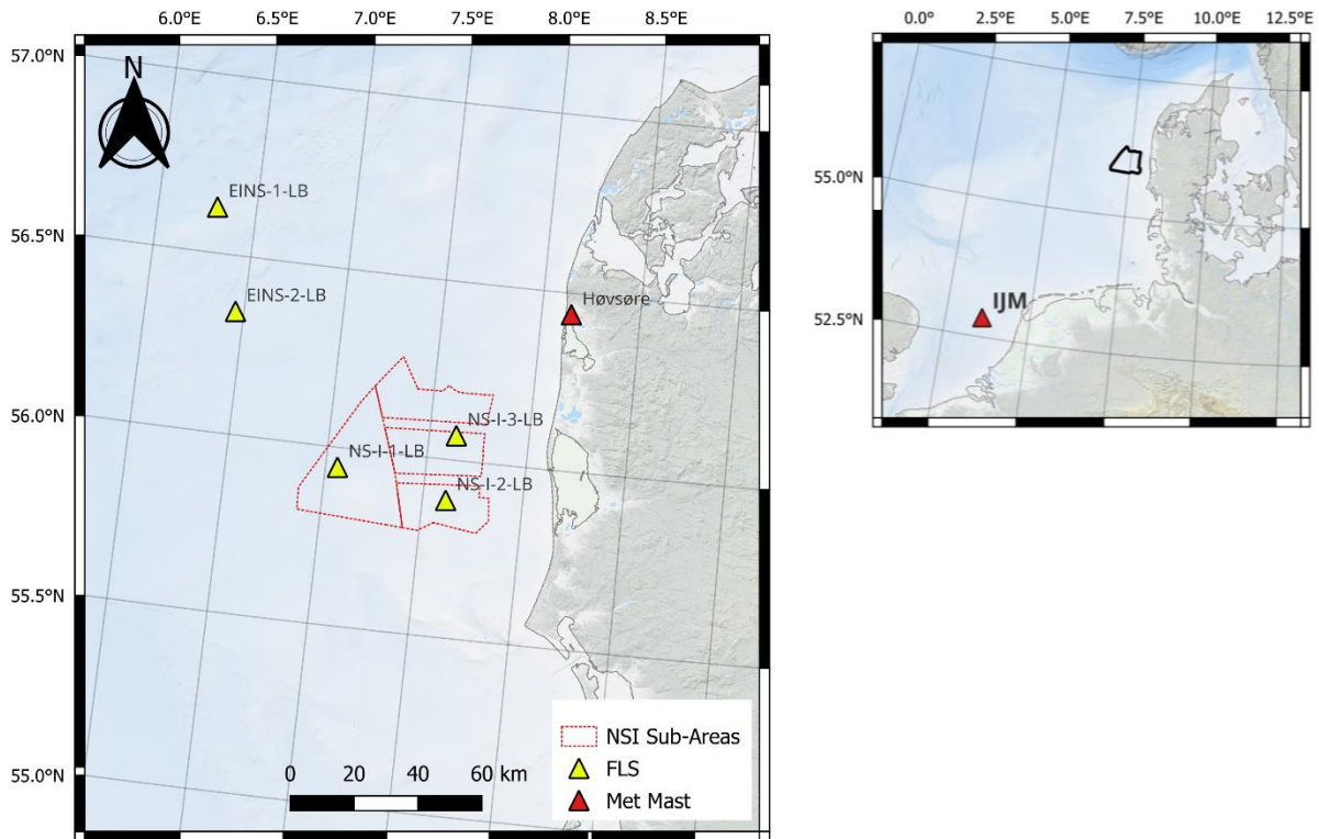
Figure 3-1: Location of the main measurement datasets used in this document. The smaller image to the right shows the location of the IJmuiden met mast. CRS: WGS84.
