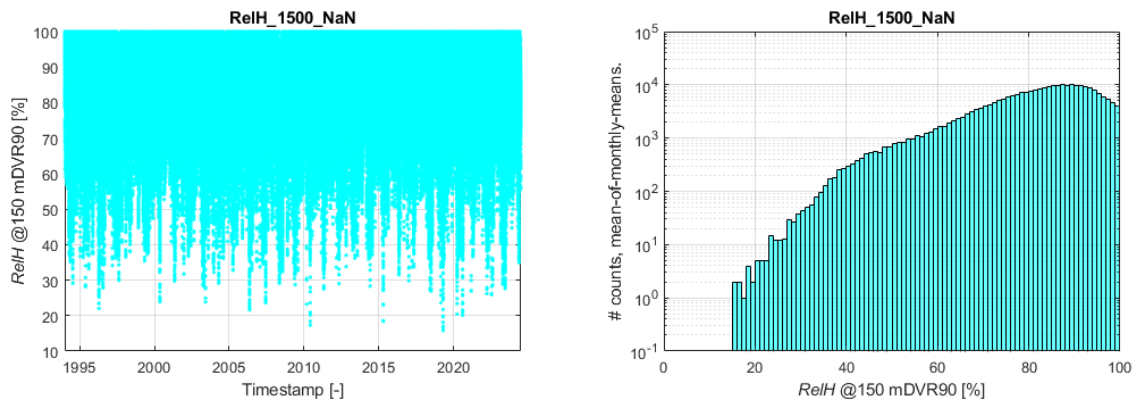
Figure 6-12: The left part of the figure shows the time series of the hourly mean values of relative humidity at 150 mDVR90 from the Vortex mesoscale dataset at the NSI-LB-3 location. The figure on the right shows an MoMM histogram of the modelled values with logarithmic 2 nd axis.
