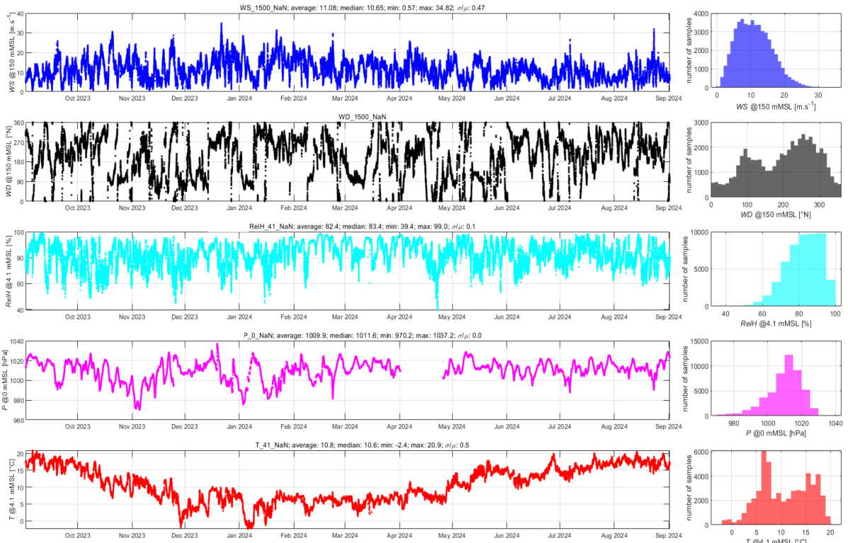
Figure B-2: Time series of wind speed and wind direction at 150 mMSL, as well as surface level air temperature, relative humidity and air pressure collected at NSI-1-LB.
