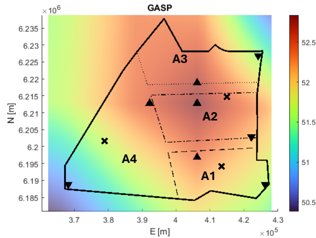
Figure 5-4: Spatial variation of 10-minute wind speed with a 50-year return period at 150 mMSL, from the GASP dataset. The coloured background follows the colour scale on the right. The highest value found within each sub-area is marked with an upwards-pointing triangle, the lowest value with a downwards-pointing triangle, and the locations of the 3 FLSs as crosses. CRS: WGS84 / UTM Zone 32N.
