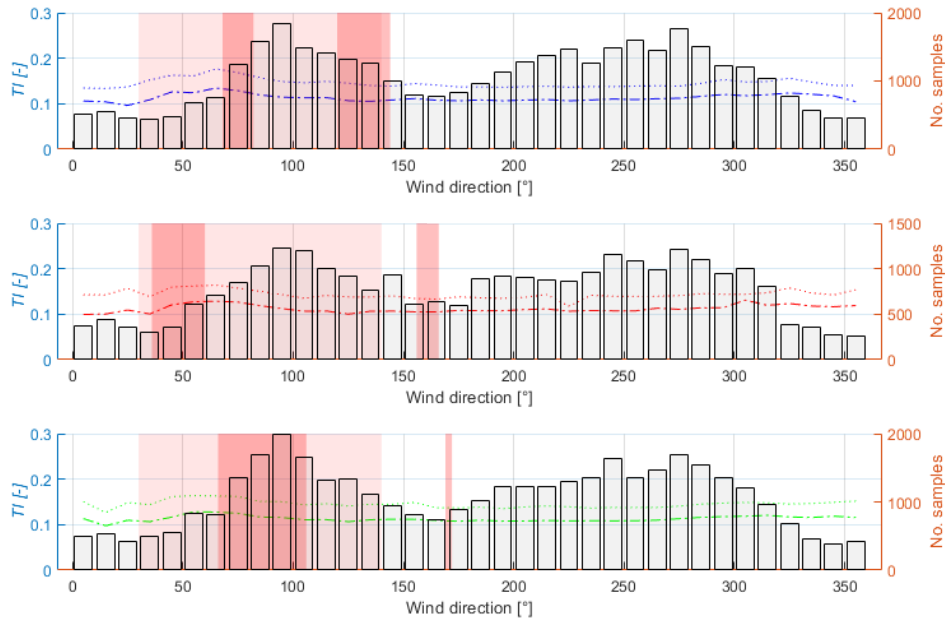
Figure 6-6: Reproduction of the plots from Figure 6-5, removing the point clouds and adding histograms to indicate the amount of data points in each directional bin example.
