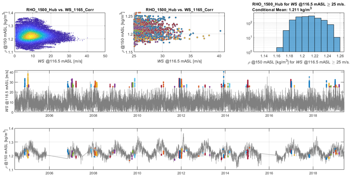
Figure 8-2: The same as Figure 8-1, but created using data from the Høvsøre met mast. Density has been extrapolated to hub height as described in Section 6.4.4, while wind speed measured at the top anemometer has not been extrapolated and is used directly.
