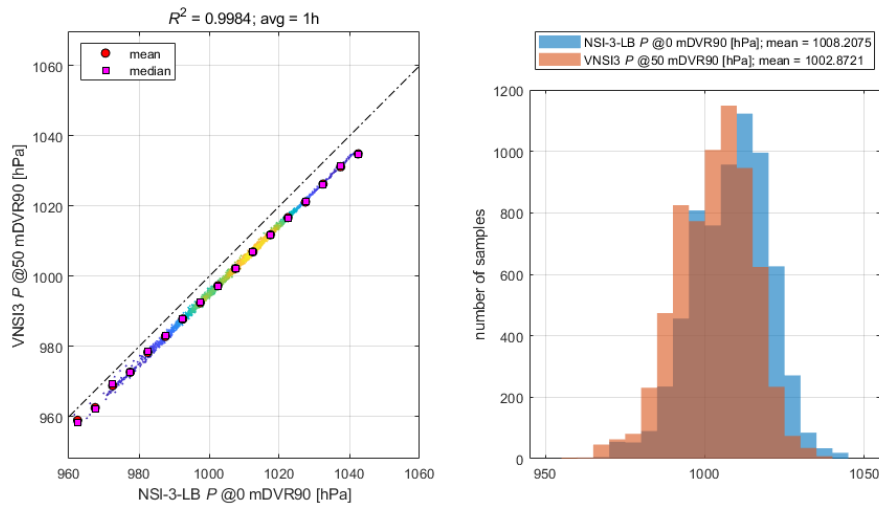
Figure 6-13: Scatter plot and histograms between atmospheric pressure measured by NSI-LB-3 at 4.1 mSWL and from the co-located Vortex model at its lowest elevation, 50 mMSL.
