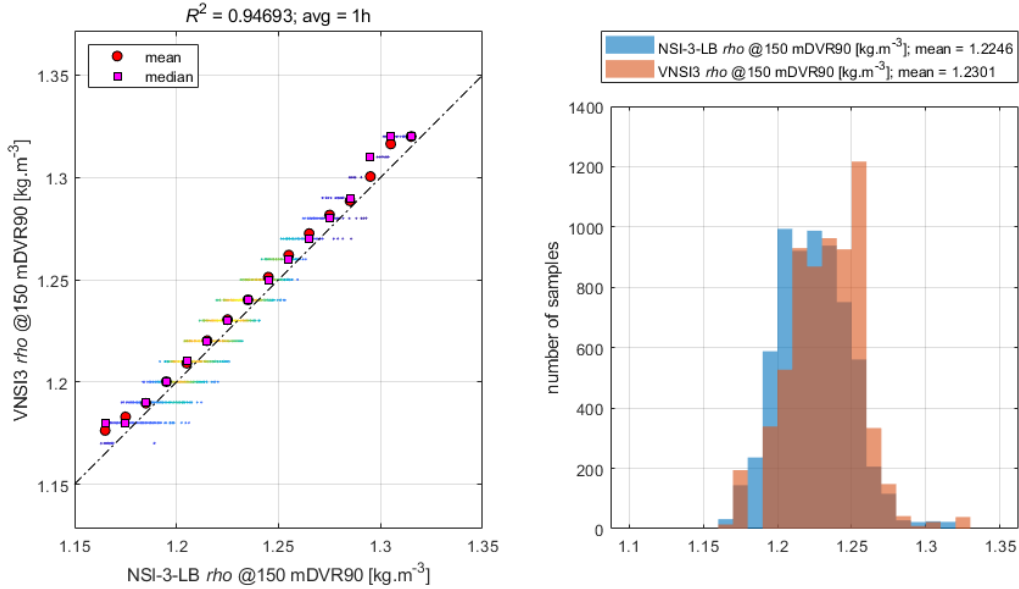
Figure 6-16: Scatter plot and histograms between air density at hub height derived from NSI-LB-3 measurements as explained in the text, and modelled by the co-located Vortex model at hub height.
