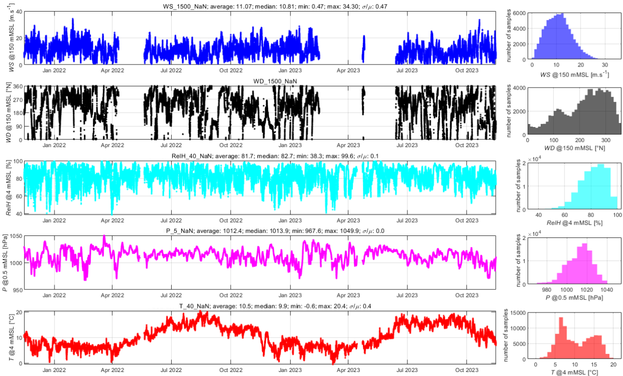
Figure B-7: Time series of wind speed and wind direction at 150 mMSL, air temperature, relative humidity and air pressure collected at EINS-1-LB.
