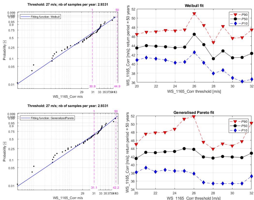
Figure 8-4: Left column: examples of distribution fits to the extreme wind speed values. Right column: results from the Extreme Value Analysis for various wind speed thresholds using the same distribution as on the left. Top row: Weibull distribution. Bottom row: Generalised Pareto distribution. Please note that these figures show the analysis without taking into account the possible missing peak measurements during the storm Bodil – see the text for how this storm is taken into account in the results of the present section.
