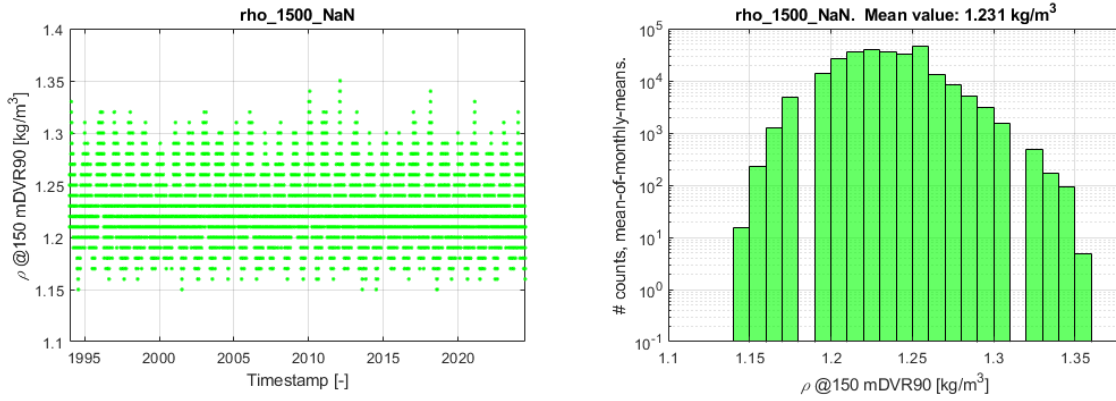
Figure 6-15: Air density at 150 mDVR90 from the Vortex time series computed at the NSI-LB-3 location. The left part of the figure shows the model time series, and the right part of the figure shows an MoMM histogram of the model values with a logarithmic 2 nd axis. The MoMM mean value is shown in the title above the histogram.
