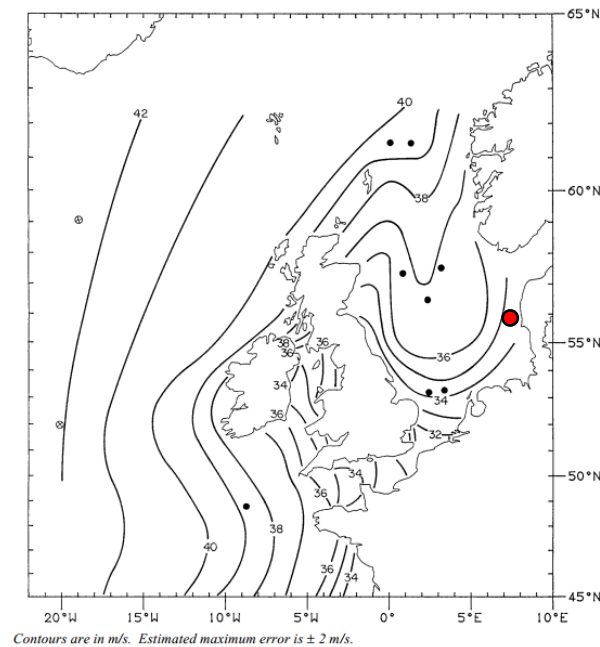
Figure 8-3: Contours of 50-year 1-hour mean 10 mMSL wind speed over Northern Europe, from Figure 1 of [UKHSE]. According to Section 3.3b) of ibid. , the values can be converted to 10-minute mean values at 10 mMSL as described in the text, and using Section 3.3c) of ibid. , the value can be extrapolated to 140 mMSL, and further extrapolated to 150 mDVR90 using the shear exponent in Section 8.1. The location of the project site is shown with a red circle. CRS: WGS84.
