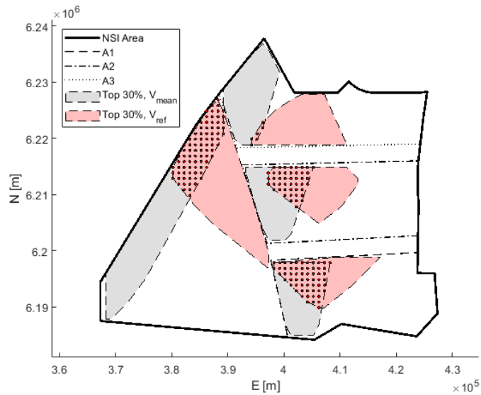
Figure 5-5: NSI area and subdivisions with the locations of the highest 30% mean wind speed (grey) and extreme wind speed (red). The representative analysis points for each subdivision are defined from the intersection of both areas. CRS: WGS84 / UTM Zone 32N.
