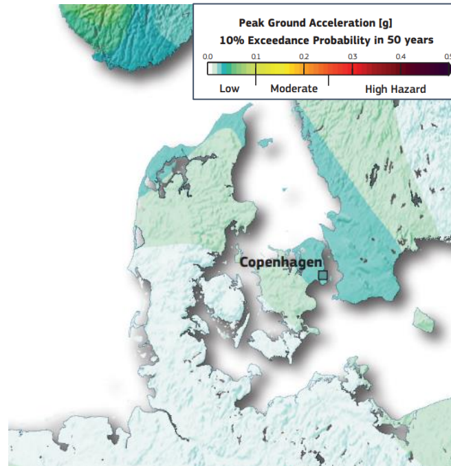
Figure 9-1: Map and colour bar showing the 475-year return period PGA, extracted from the [SHARE] database. Note that the values are in units of g , yielding a PGA interval at the site of <0.25\text{-}0.29 \text{ m/s}^2 .
