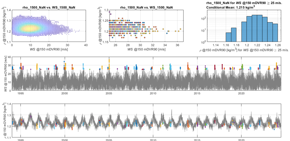
Figure 8-1: Plots for determining the air density for high wind speeds. The scatter plot on the top left shows all air density data from the Vortex time series at 150 mDVR90 vs. wind speed at 150 mDVR90, where the colours show the density of points. The plot at the top in the middle shows a detail of the figure on the left for WS \geq 25 m/s, but the colours here show the timestamp so that similar colours show events that are close in time. By careful study of this figure, one can see that the points with the very strongest wind come from only a single event, which is why wind speeds down to 25 m/s have been included in order to capture data from several storms. The top rightmost part of the figure shows a histogram of the data in the plot in the middle, and its title shows the mean value of these air densities. Graphs of the 150 mDVR90 wind speed and -air density time series are shown at the bottom of the figure, where the coloured points correspond to the events shown in the middle figure on the top.
