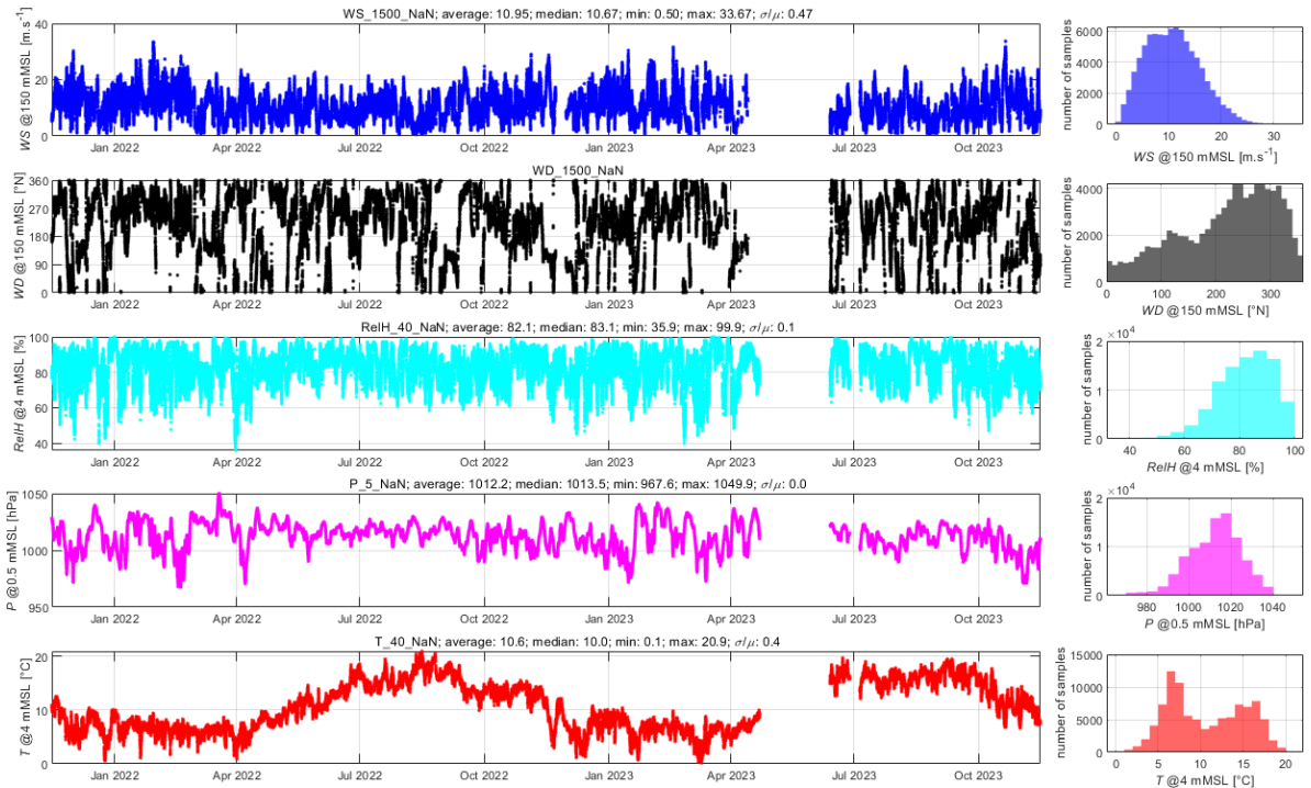
Figure B-8: Time series of wind speed and wind direction at 150 mMSL, air temperature, relative humidity and air pressure collected at EINS-2-LB.
