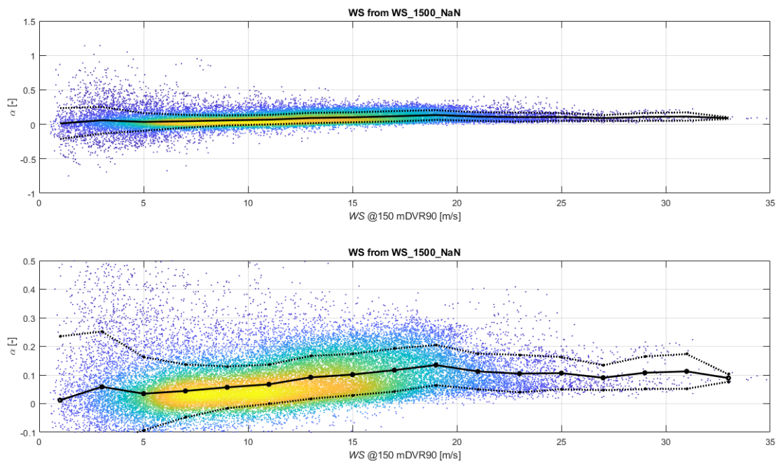
Figure 6-3: Scatter plots of wind shear exponents vs. hub height wind speed, obtained from the hub height sensor at the NSI1 FLS and fitting the wind profile across all elevations covering the rotor plane and up to 300 mMSL as listed in Section 1.2. The plots show the points coloured according to density. The upper plot shows all data, whereas the lower plot shows details for the most widespread values. The black points, joined by the fully drawn black line, show the mean-of-monthly means wind-speed binned mean values. The markers joined by dashed lines show the mean values described in the preceding sentence, plus and minus one mean-of-monthly-means wind speed binned standard deviation.
