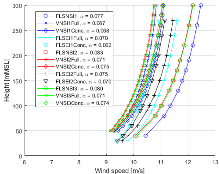
Figure 6-2: Mean wind speed profiles and fitted shear exponents to the 3 NSI FLSs, their co-located Vortex model time series, and the 2 EINS FLSs.
