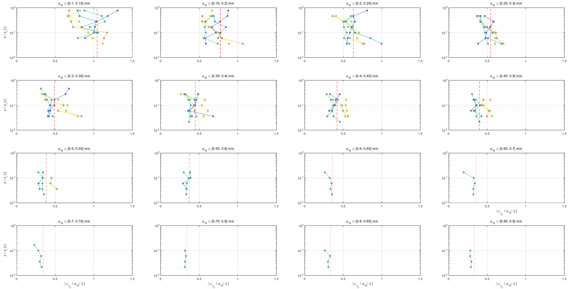
Figure C-7: Using the same colour code as in Figure C-6, this figure shows mean ratios of \sigma_{\sigma_U}(z)/u_{*0} and the model results (Eq. C-8) with dashed red lines.
