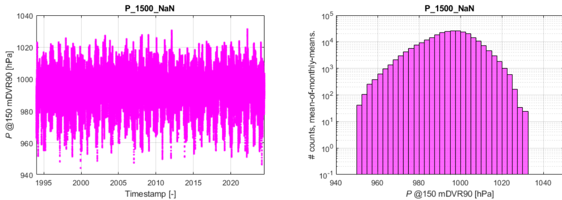
Figure 6-14: The left part of the figure shows the modelled time series of air pressure at 150 mDVR90 from the Vortex mesoscale dataset at the NSI-LB-3 location. The right part of the figure shows an MoMM histogram of the modelled values with a logarithmic 2 nd axis.
