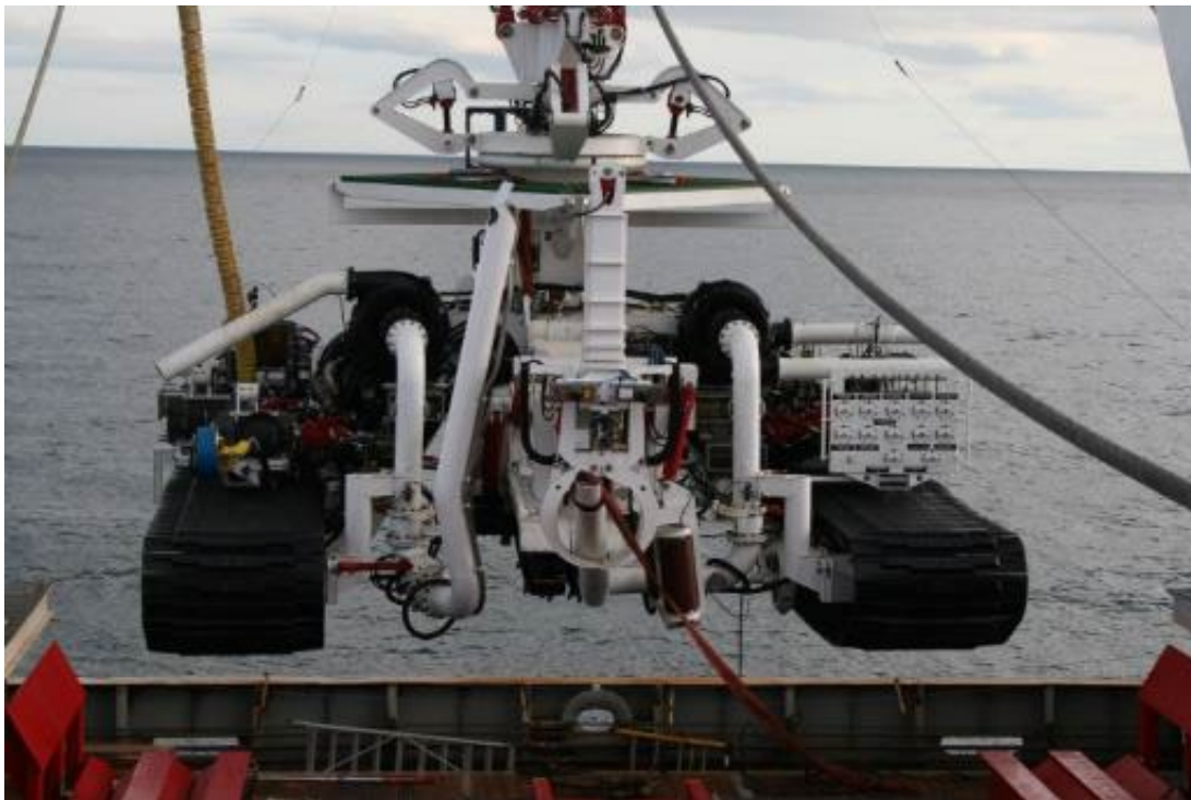
Helix Robotics I-trencher
