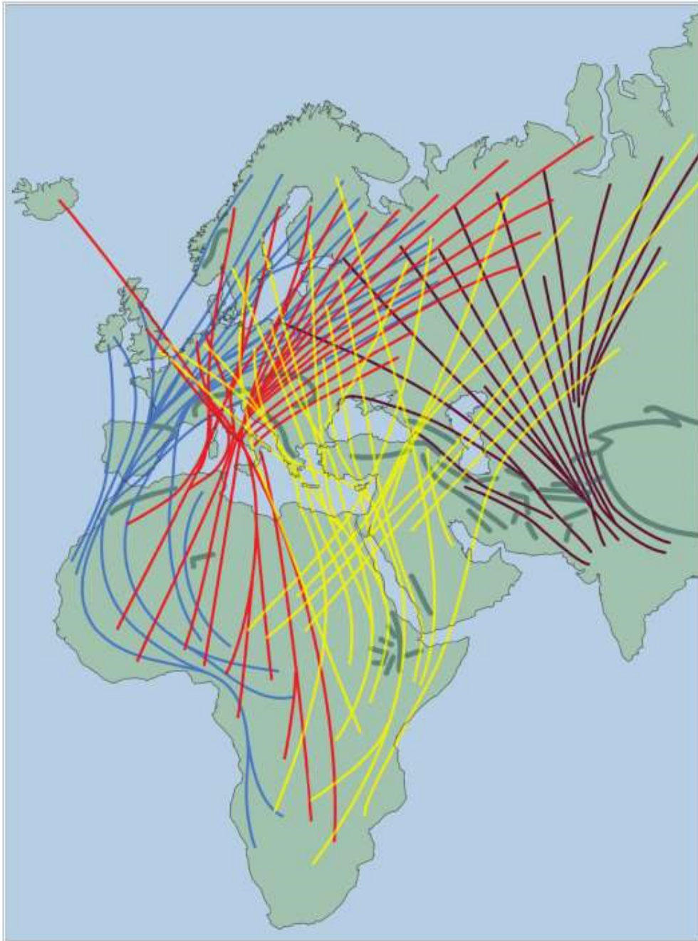
Figure 3-5: The four main fly way routes occurring in the Paelearctic: 1) the western/Atlantic (blue), 2) the Central (Apennine, red), 3) South-Eastern (Balkan, yellow) and 4) Eastern (Indian, brown). Taken from Busse et al., 2014.
